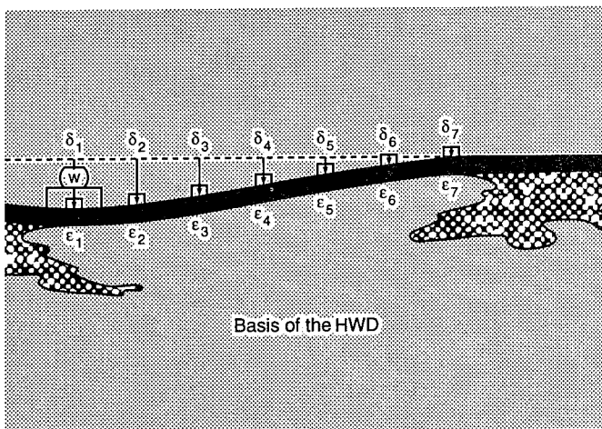
Figure 4. Basis of HWD testing.
