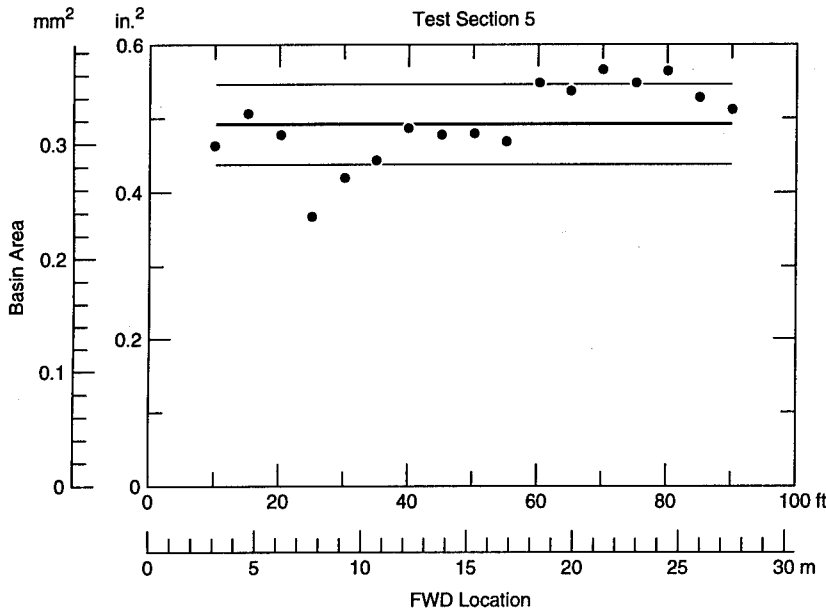
Figure 17. Deflection basin area for 2% RSB.
