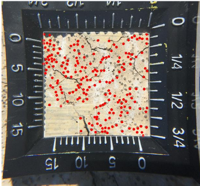
Figure 19: Sample Magnification Area with Bead Loss Count in Red
