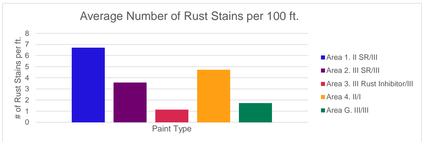
Figure 33: Average Number of Bottom-Up Rust Spot Stains per 100 ft
