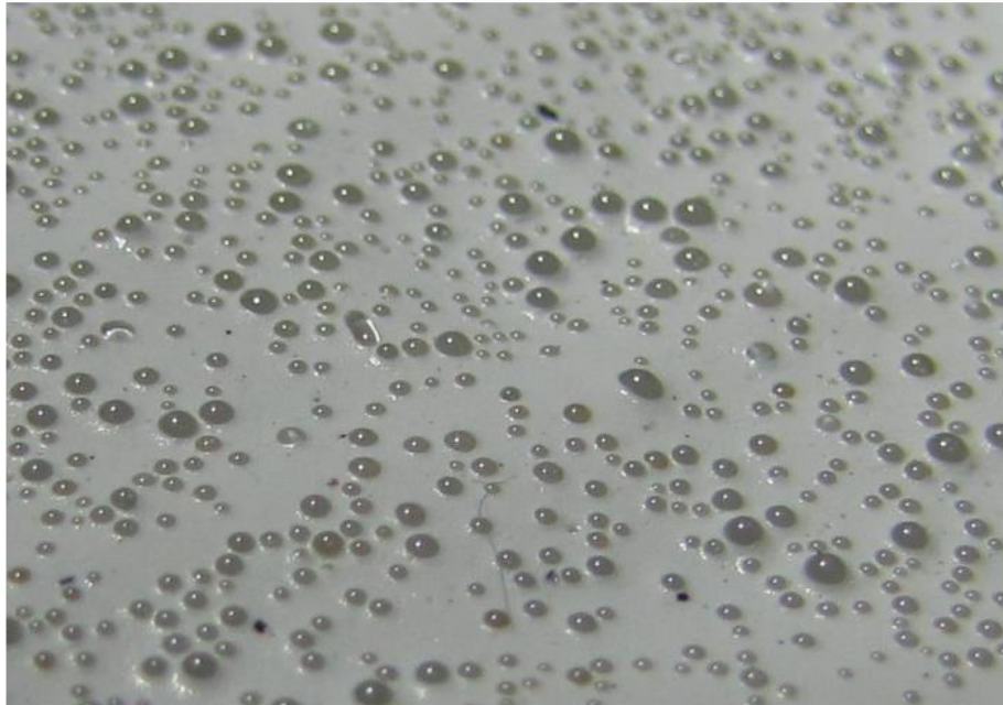
Picture 8 – close up of 25 mil Type III, stain resistant paint with Type III beads at 10# per gallon.
