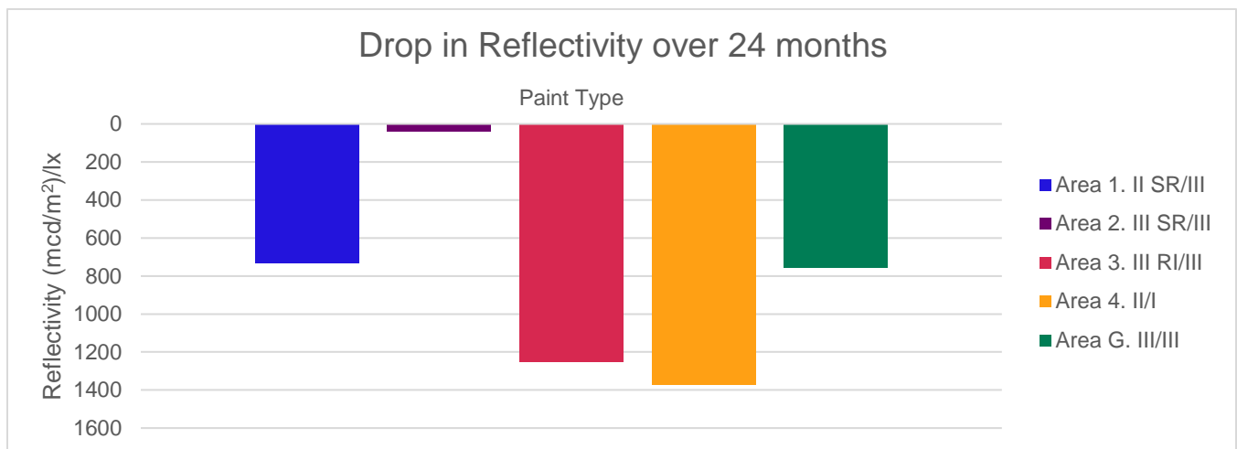
Figure 35: Drop in Reflectivity over 24 months
