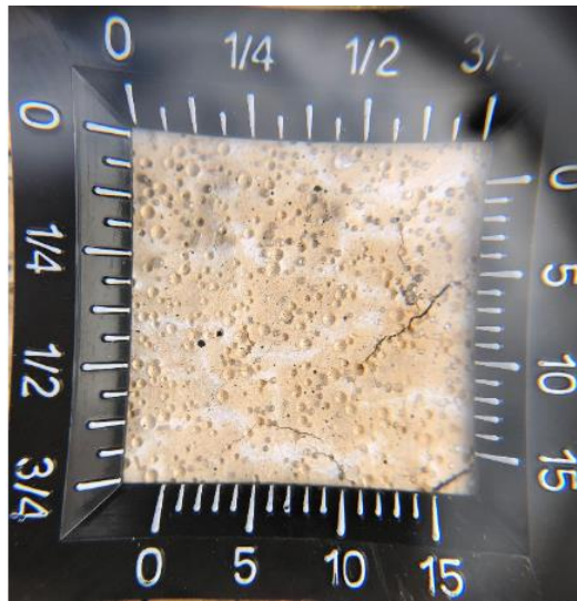
Figure 37: Area G - Sample 1A – 12/5/2017
