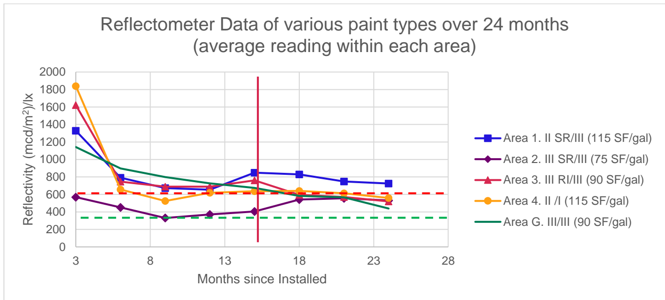
Figure 34: Average Reflectometer Readings
