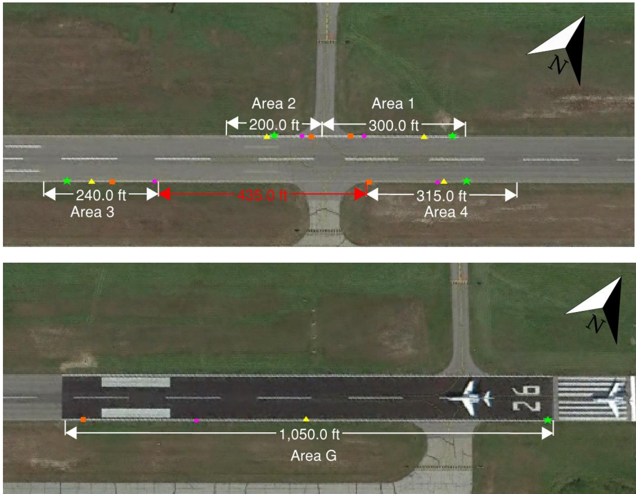
Figure 14: Locations of Random Sampling Within Each Study Area
