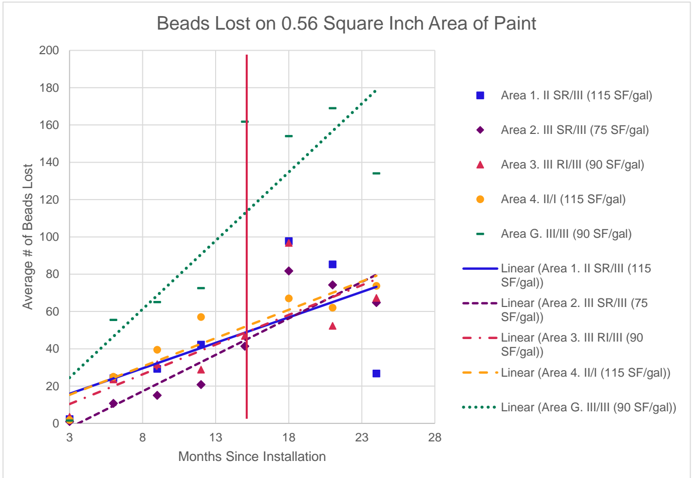
Figure 36: Average Bead Loss per Area
