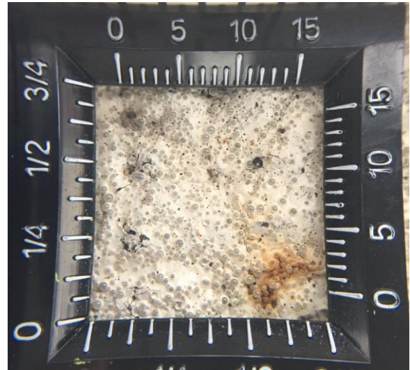
Figure 4: Bead Loss Counting Photograph
