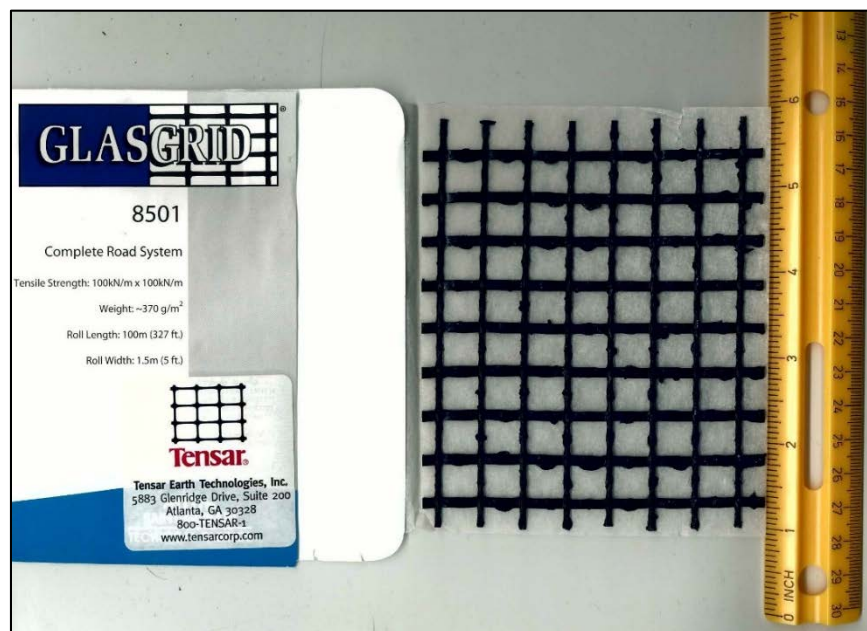
Figure 2. A photograph of GlasGrid fiberglass mesh installed in NH 101.
