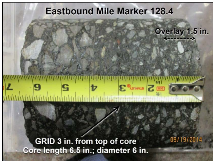
Figure 21. Asphalt core for EB MM 128.4.
