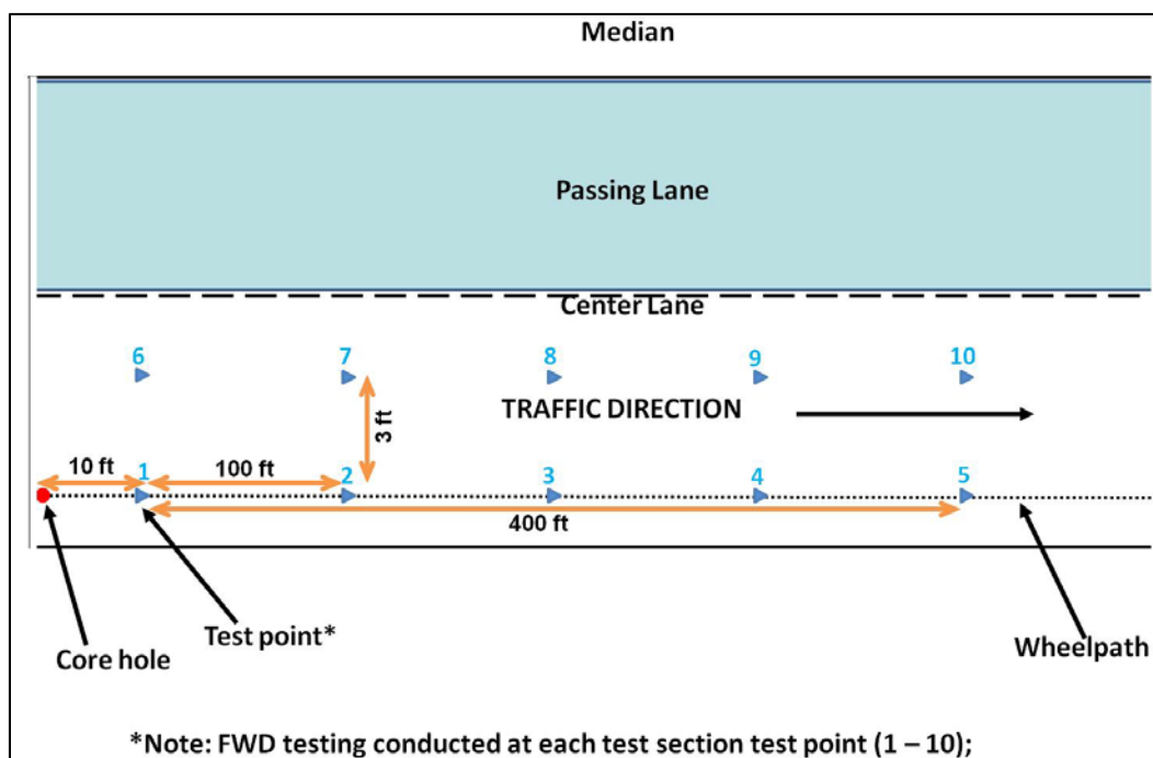
Figure 14. Test section layout at all mile markers, except at WB MM 131.5 where testing was conducted in the passing lane.
