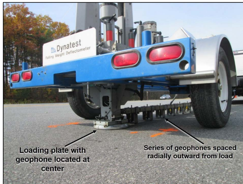
Figure 17. Test section WB MM 128.0 FWD testing showing loading plate and proximity of geophone spacing on the pavement surface.
