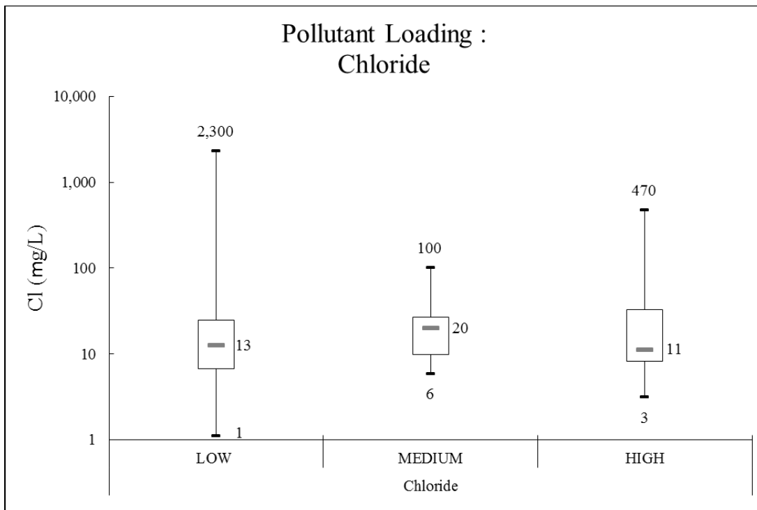
Figure 9: Box and whisker plot of Chloride (Cl) results for each of the monitored locations.
