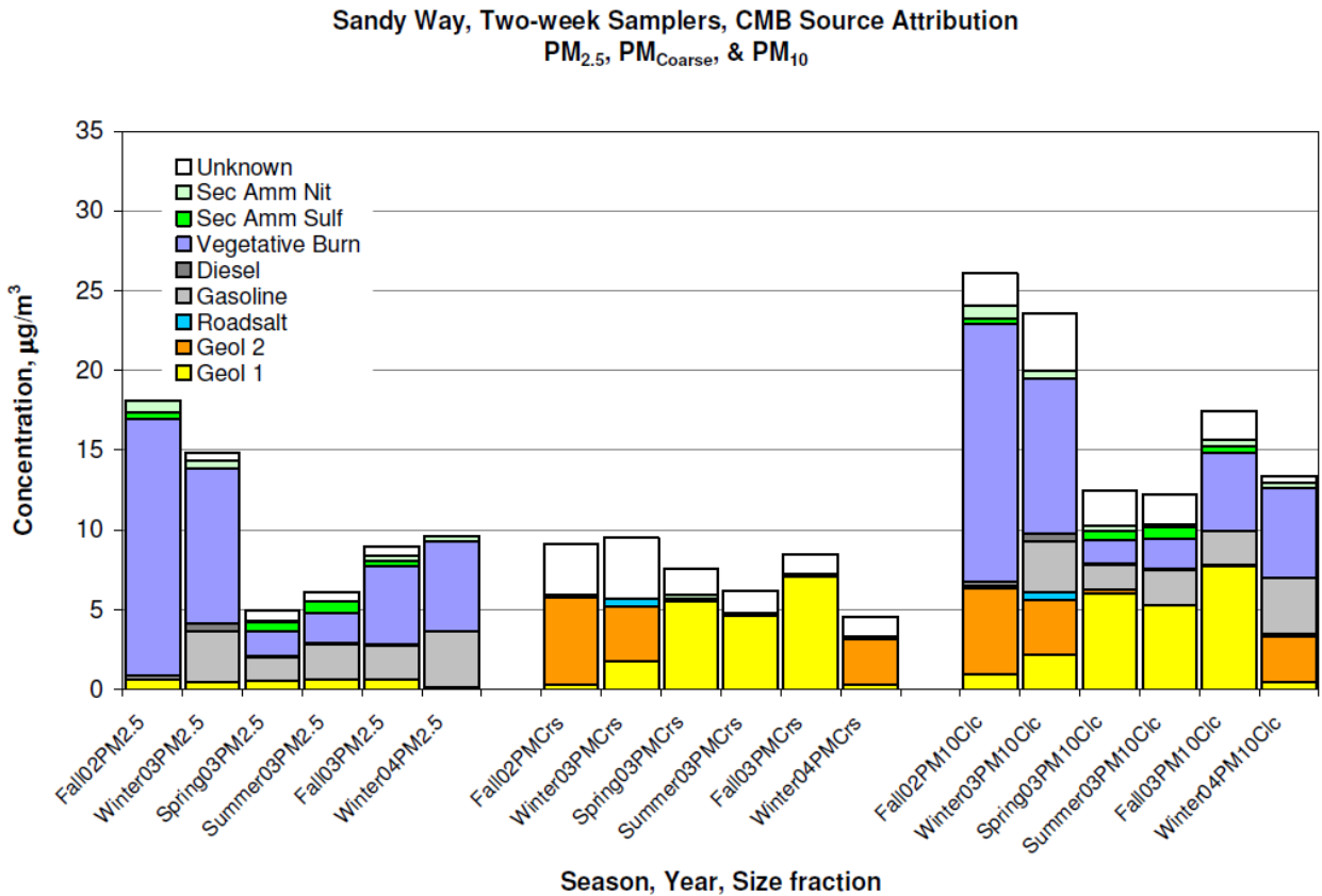
Figure 3: Lake Tahoe Source Attribution Study (Ref. 7) chart displays the various sources of particulate matter (PM) broken down by size fraction (PM 2.5 , PM coarse , PM 10 ) and season. Samples taken at the Sandy Way project site over a two week period.
