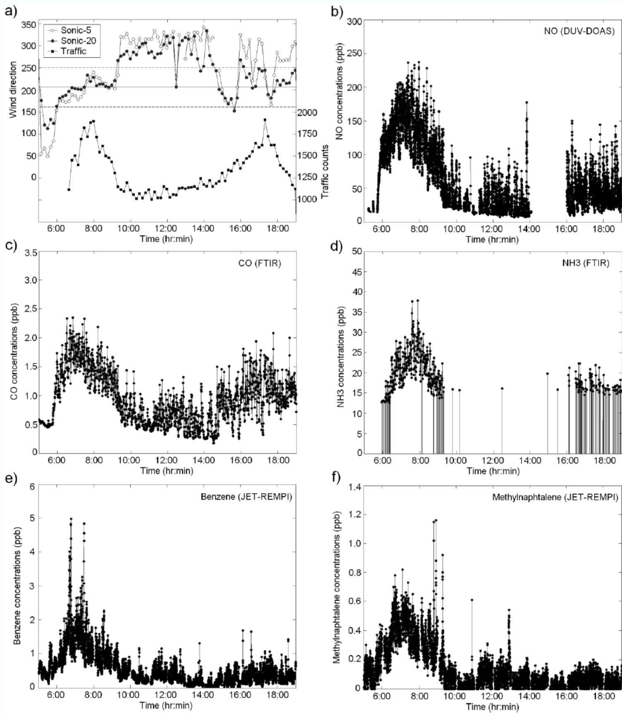
Figure 2: Comparison of measurements from on-site instrumentation (i.e. DUV-DOAs, FTIR, and Jet-REMPI) for August 3, 2006 for (a) wind direction, (b) NO, (c) CO, (d) NH 3 , (e) benzene, and (f) methylnaphthalene.
