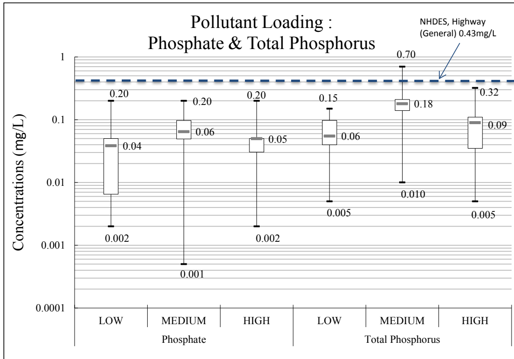
Figure 8: Box and whisker plot of Phosphate (PO 4 ) and Total Phosphorus (TP) results for each of the monitored locations. The dotted line is the EMC value for TP used in the NHDES Simple Method calculations.
