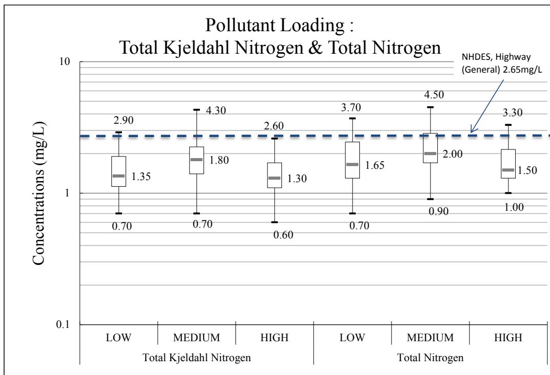
Figure 7: Box and whisker plot of Total Kjeldahl Nitrogen (TKN) and Total Nitrogen (TN) results for each of the monitored locations. The dotted line is the EMC value for TN used in the NHDES Simple Method calculations.
