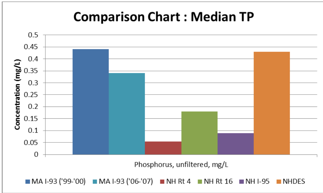
Figure 13: Comparison of median total phosphorus (TP) values from Massachusetts Interstate 93, New Hampshire Route 4, Route 16, and Interstate 95, and NHDES Simple Method pollutant loading calculations.
