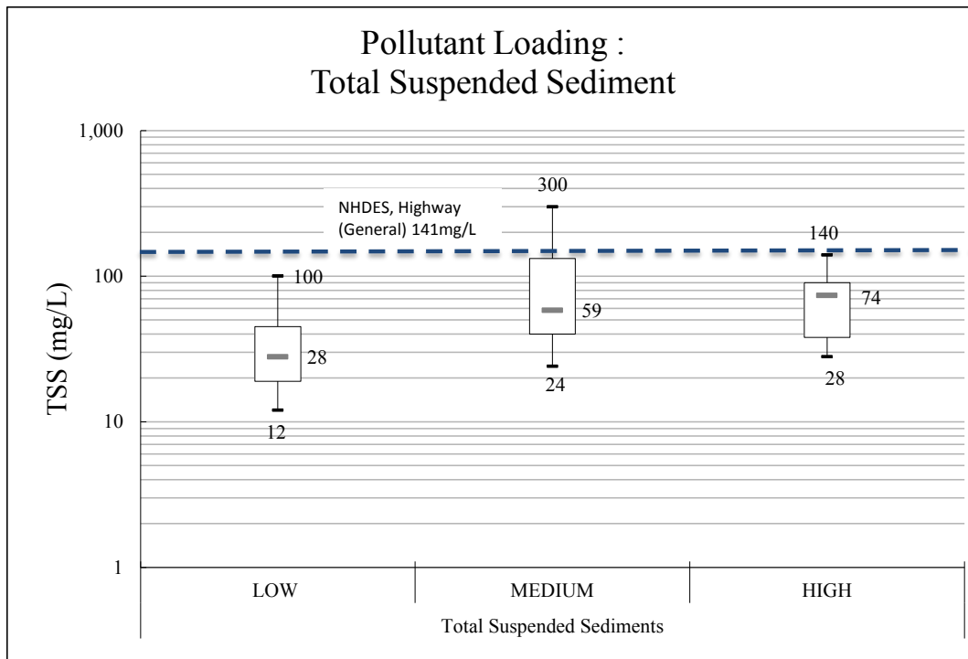
Figure 4: Box and whisker plot of total suspended sediment (TSS) results for each of the monitored locations. The dotted line is the EMC value for TSS used in the NHDES Simple Method calculations.
