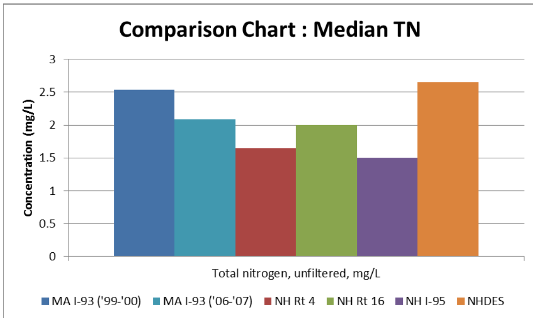
Figure 12: Comparison of median total nitrogen (TN) values from Massachusetts Interstate 93, New Hampshire Route 4, Route 16, and Interstate 95, and NHDES Simple Method pollutant loading calculations.
