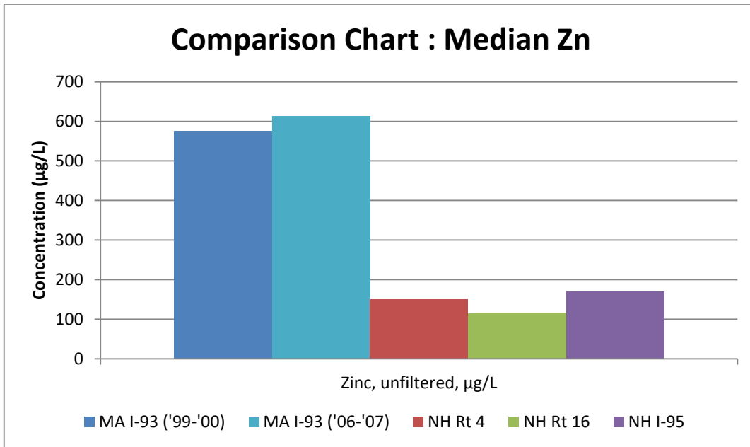
Figure 11: Comparison of median zinc (Zn) values from Massachusetts Interstate 93, New Hampshire Route 4, Route 16, and Interstate 95.
