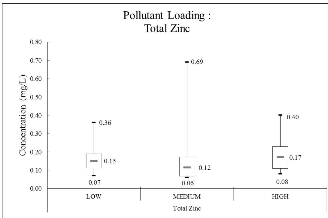
Figure 5: Box and whisker plot of heavy metal results for each of the monitored locations. Only zinc is included in this plot because copper was consistently below detectable limits of the analytical method.
