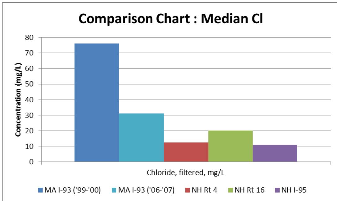
Figure 14: Comparison of median chloride (Cl) values from Massachusetts Interstate 93, New Hampshire Route 4, Route 16, and Interstate 95. (Note – NH sites only sampled in non-winter months)
