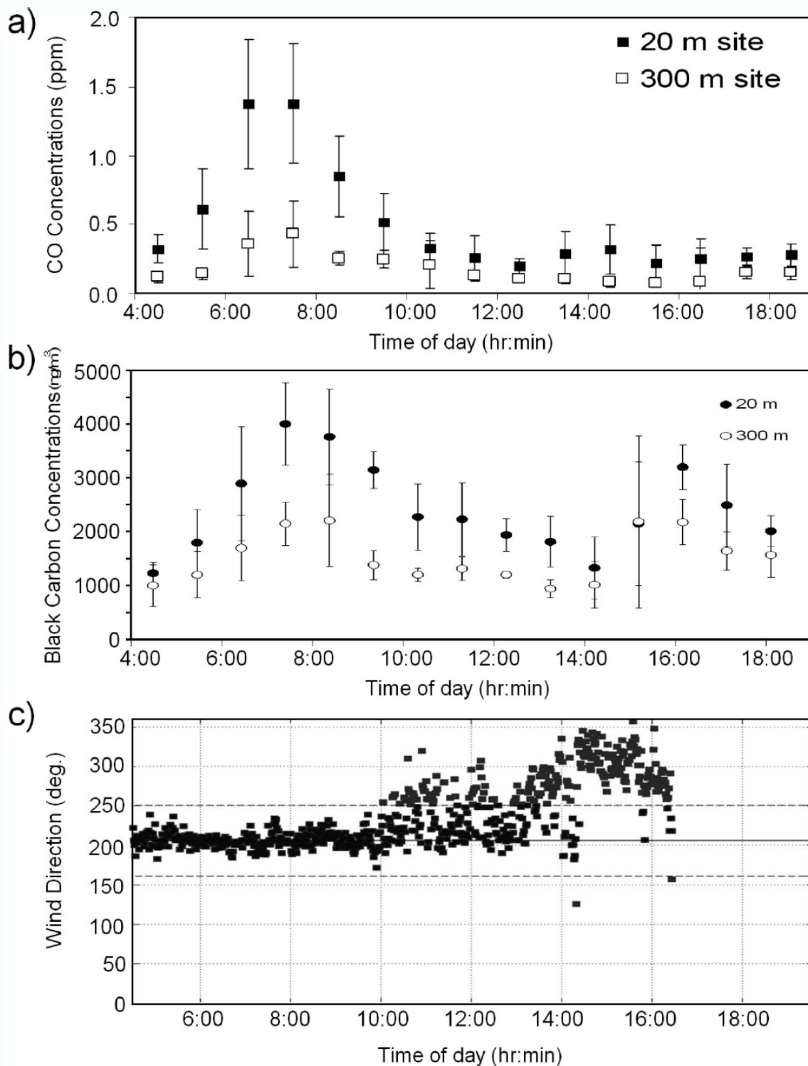
Figure 1: Comparison of (a) CO and (b) BC hourly average pollutant concentrations and measurement standard deviations by distance from the road on August 7, 2006. Panel c shows the 1-min average wind speed and direction profiles for this day on the basis of measurements from Sonic-20.6
