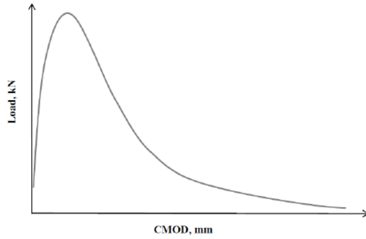
Figure 6- A Typical Load-CMOD Test Curve (Marasteanu et al., 2012)
