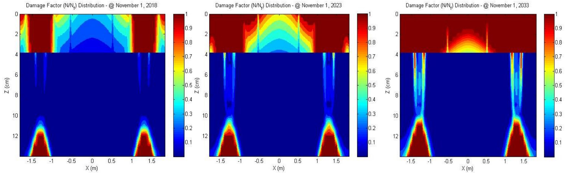
Figure 63– Plant Produced, PG 58-28, 12.5mm, 18.5% RAPRAS (Surface layer) and PG 58-28, 19mm, 20.4% RAPRAS (Binder layer) (5, 10, and 20 Years)
