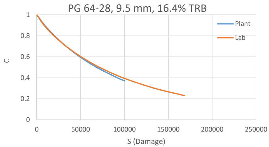
Figure 50- Damage Characteristics Curves of Hooksett Mixtures
