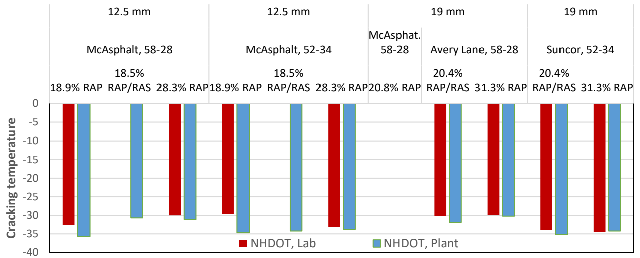
Figure 15- Cracking Temperature for Extracted and Recovered Lebanon Binders
