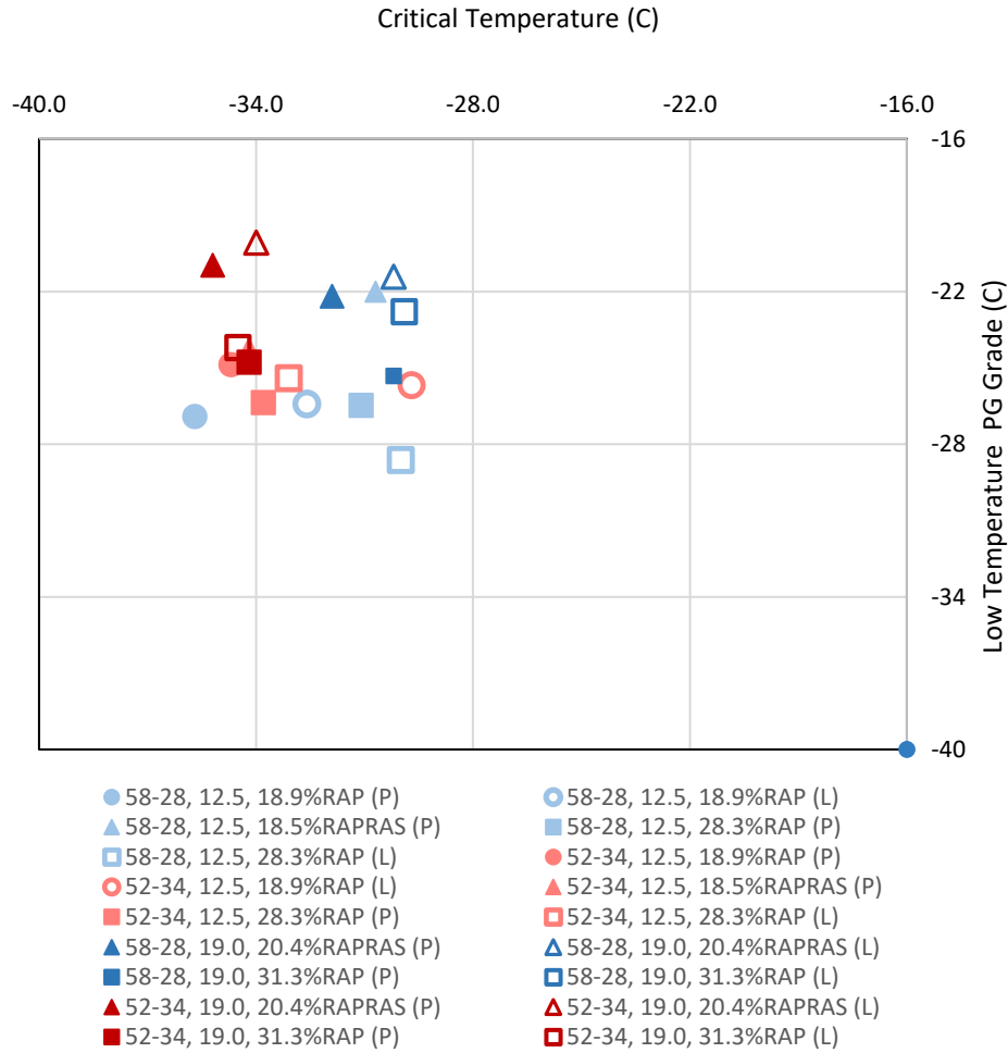
Figure 16- Critical Temperature versus Low Temperature PG Grade
