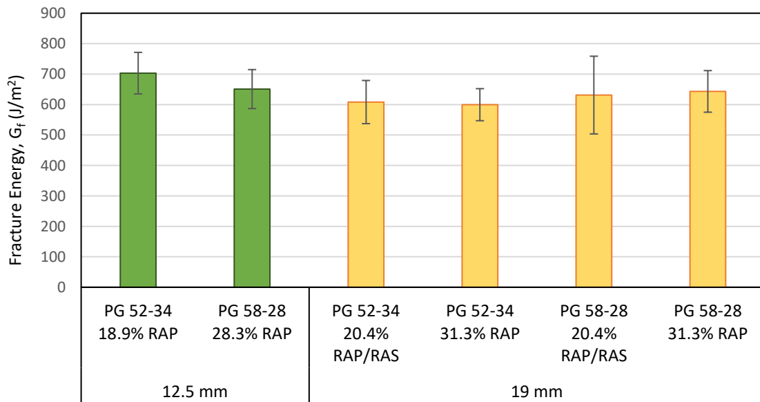
Figure 46- Average Fracture Energy of Different Mixtures
