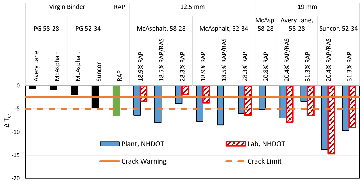
Figure 10- \Delta T_{cr} of Different Lebanon Binders
