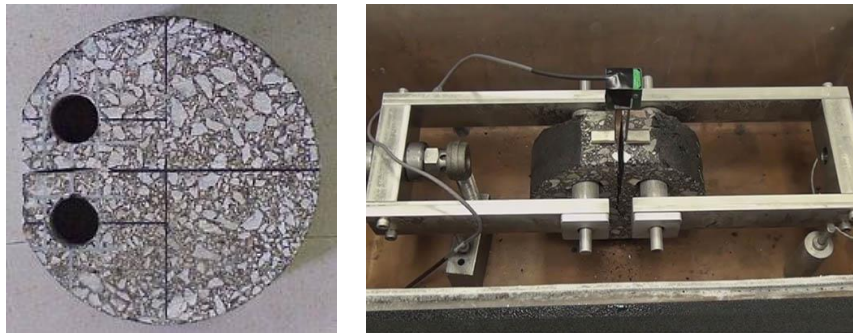
Figure 5- Disk-Shaped Compact Tension Testing Specimen and Configuration, (ICT, and Minnesota Transportation Research Blog)
