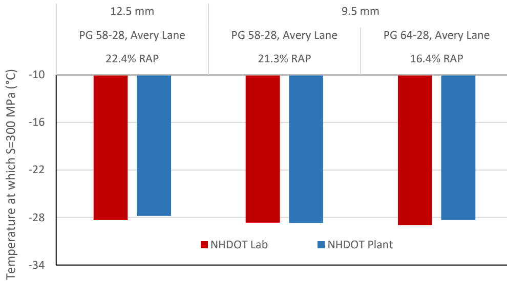
Figure 13- Critical Temperature where S=300 MPa for Hooksett Mixtures
