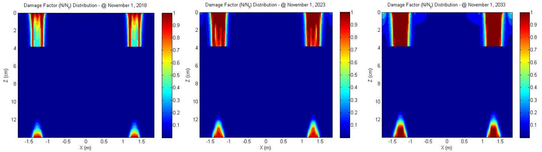
Figure 69– Plant Produced, PG 52-34, 12.5mm, 28.3% RAP (Surface layer) and PG 52-34, 19mm, 31.3% RAP (Binder layer) (5, 10, and 20 Years)
