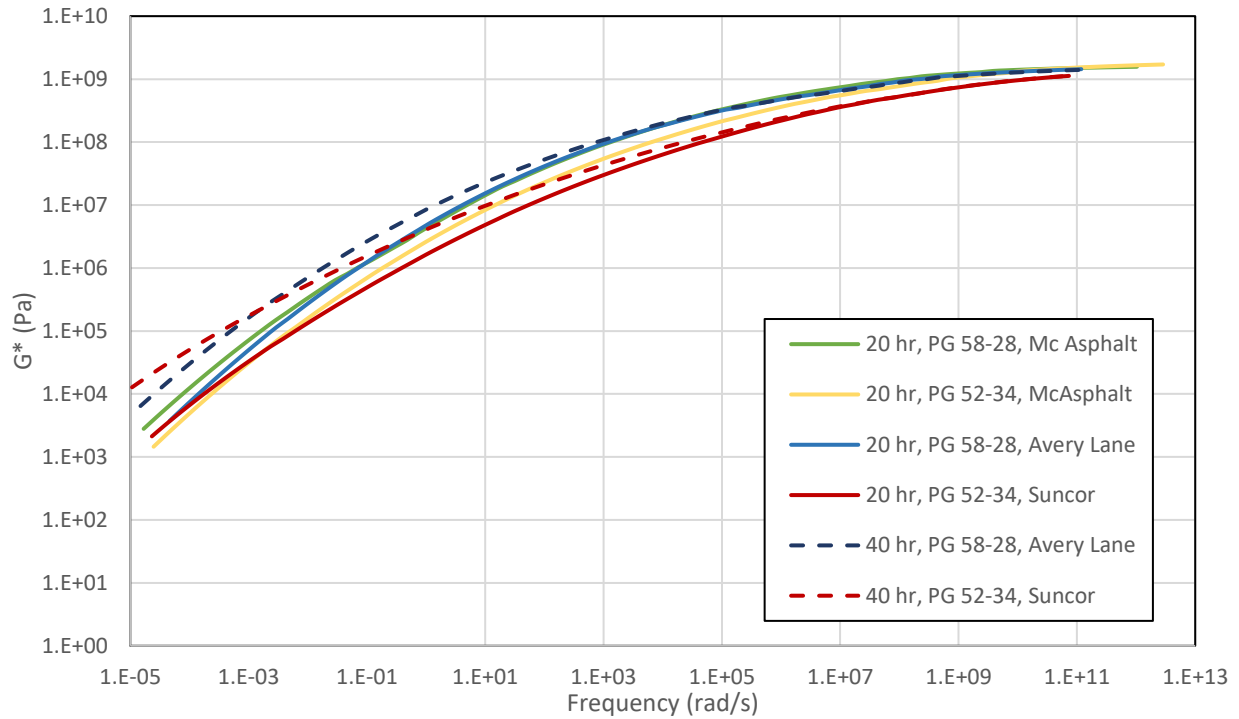
Figure 19- G^* mastercurves of virgin binders (15° C reference temperature)
