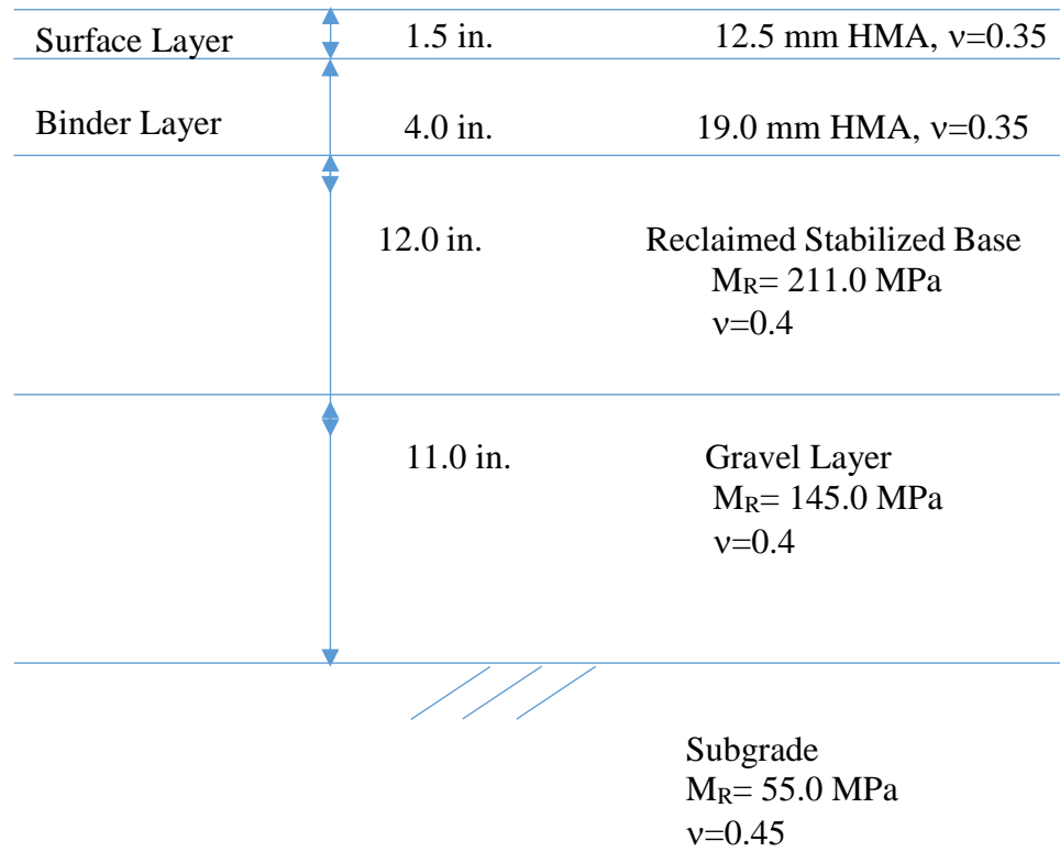
Figure 53- Westmoreland Pavement Cross Section
