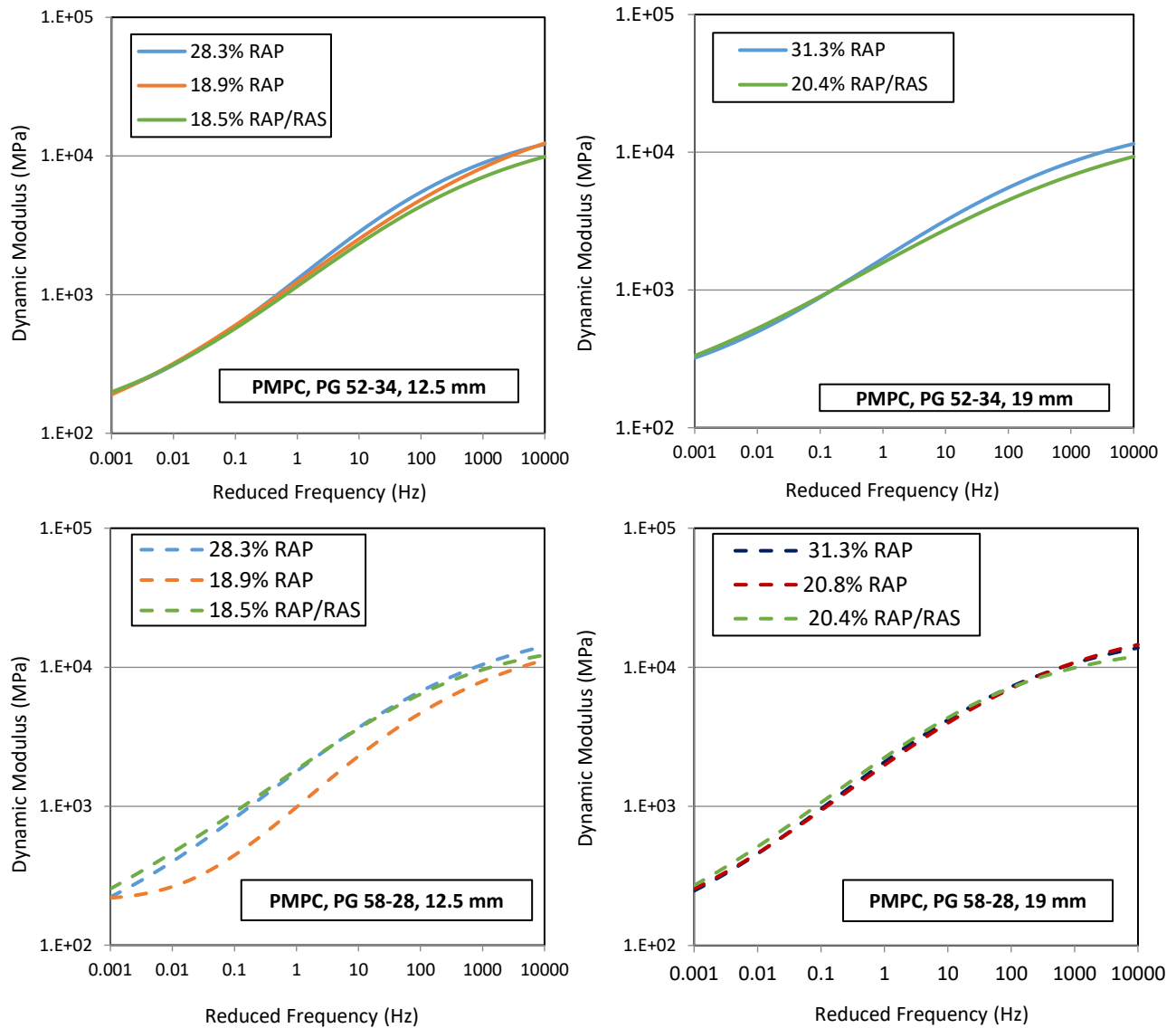
Figure 31- Dynamic Modulus Mastercurves of PMPC mixtures
