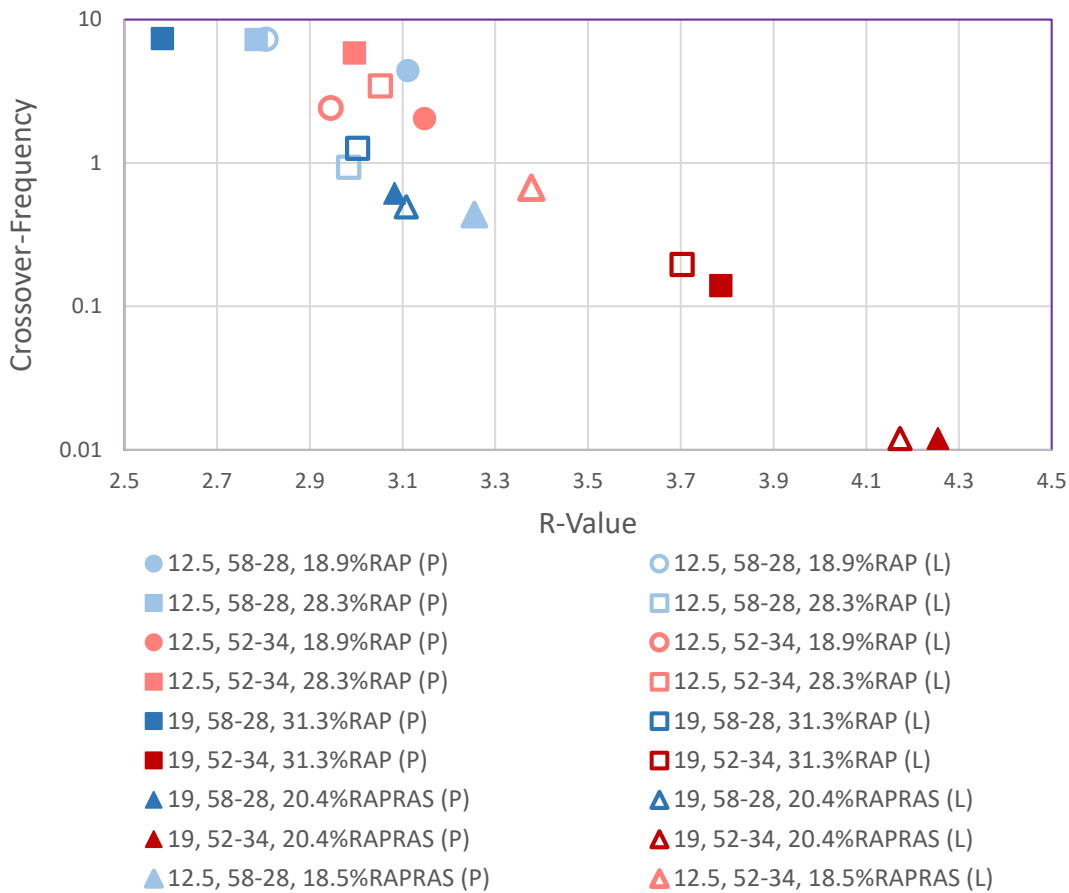
Figure 26- Crossover Frequency versus R-value for different mixtures
