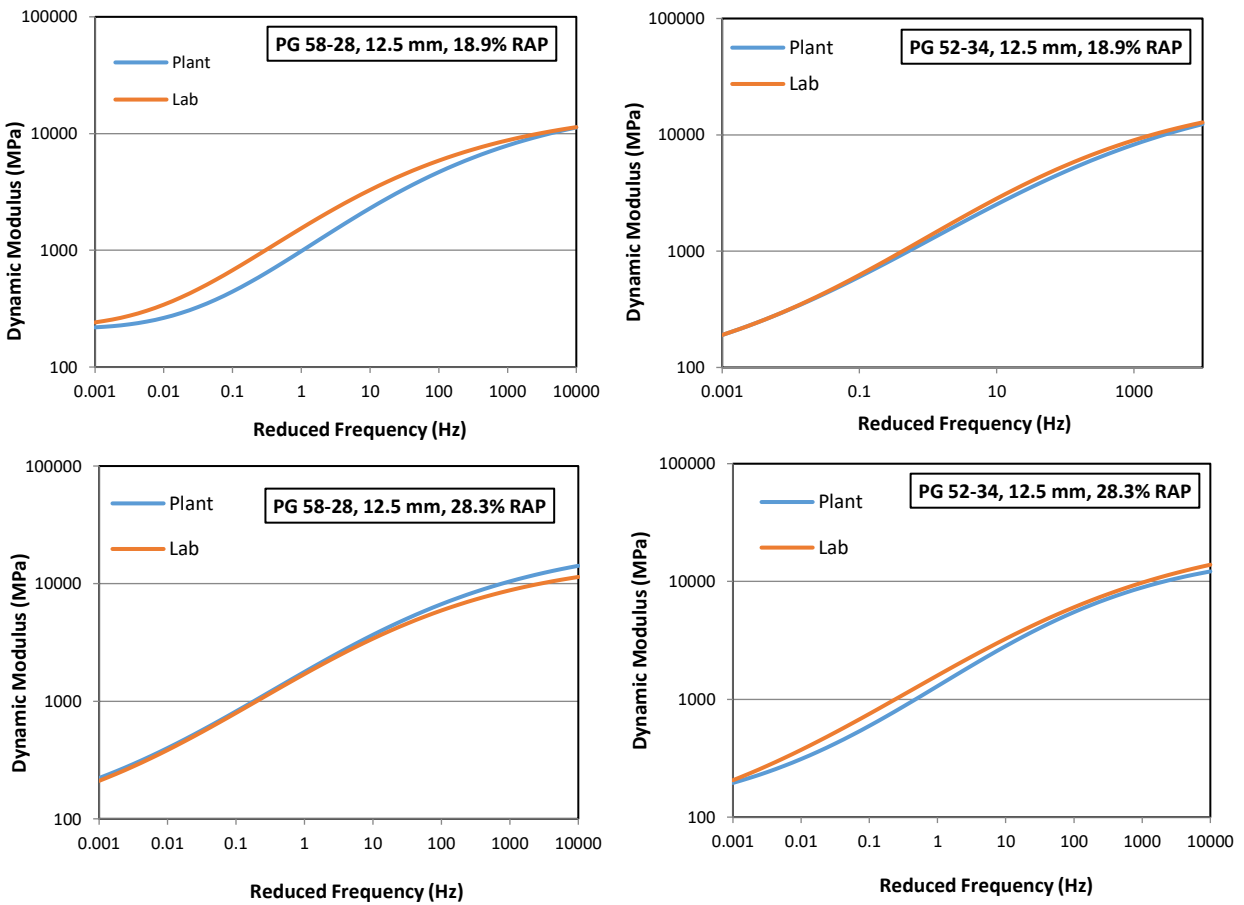
Figure 27- Dynamic Modulus Mastercurves for 12.5 mm, LMLC and PMPC Mixtures
