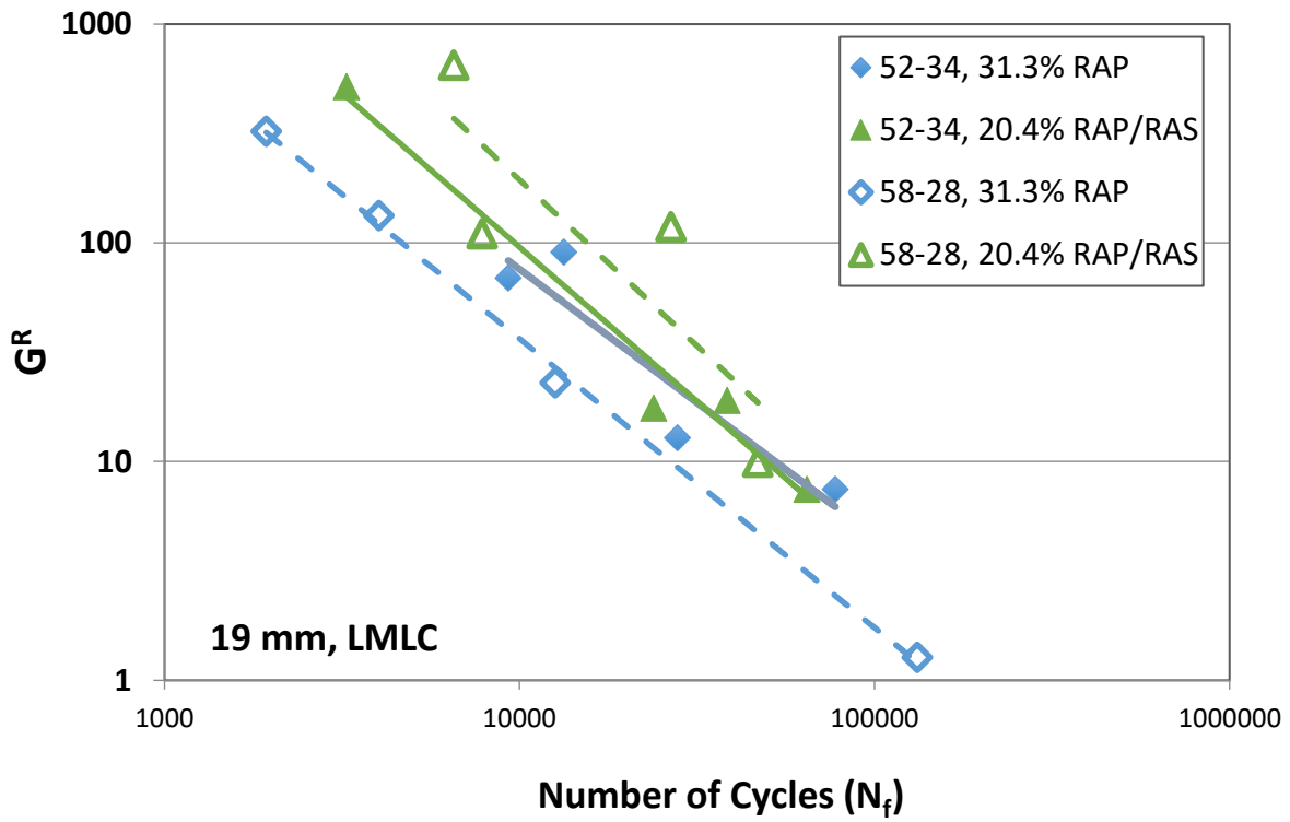
Figure 45- Fatigue Failure Diagrams of LMLC Mixtures
