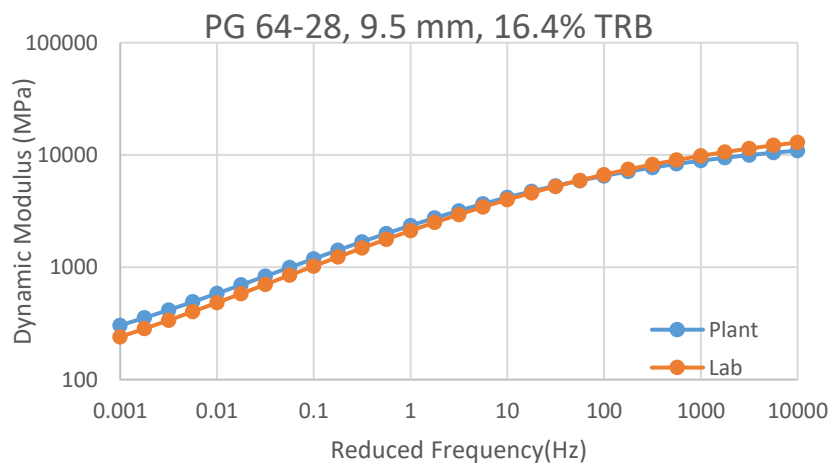
Figure 48- Dynamic Modulus Mastercurves of Hooksett Mixtures
