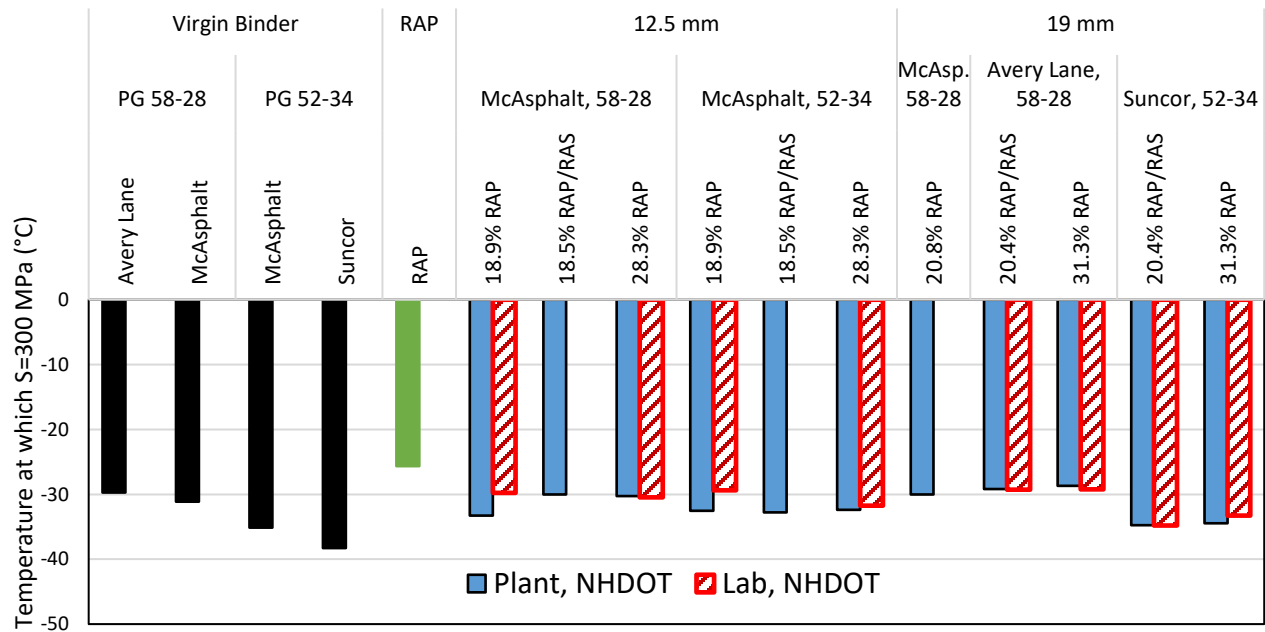
Figure 9- Creep Stiffness for Lebanon Mixtures
