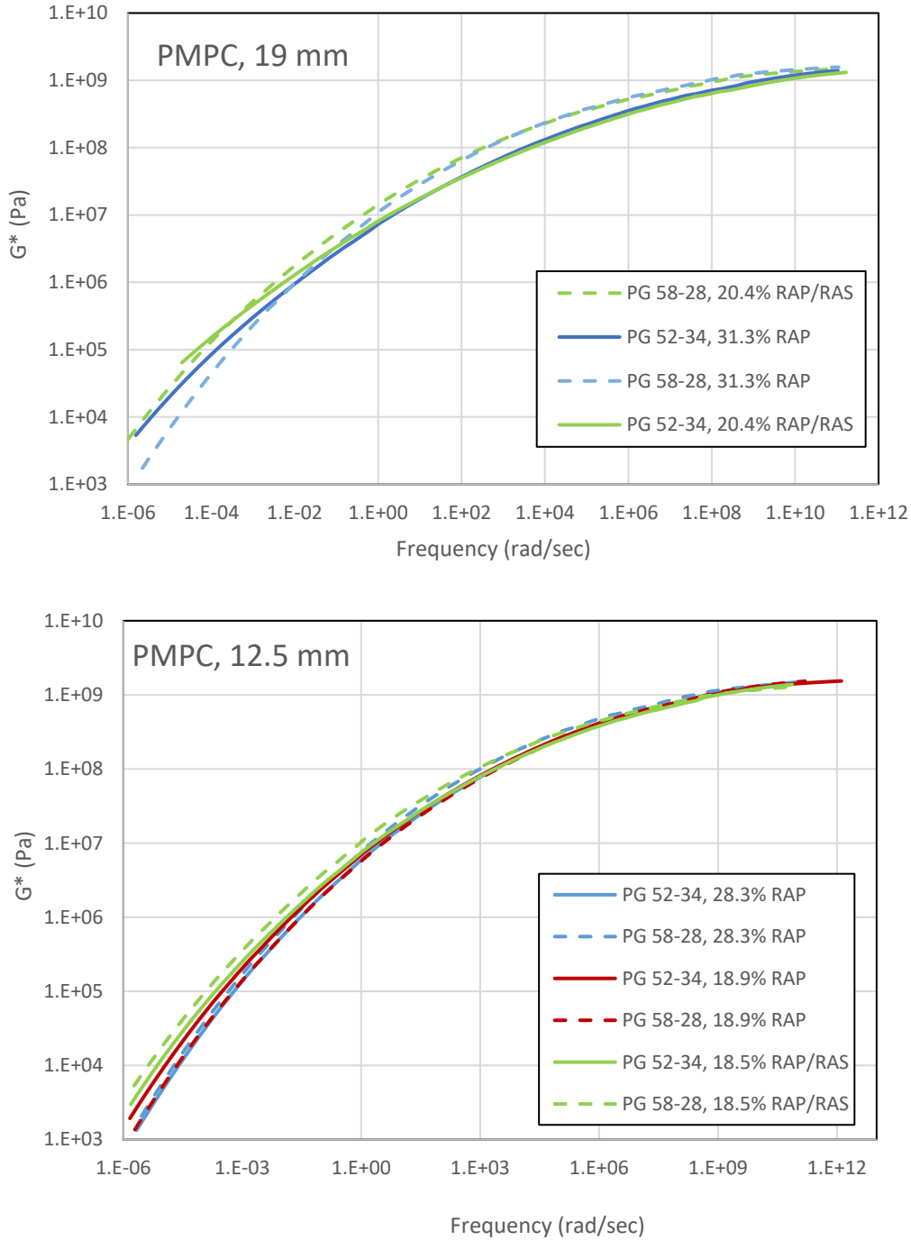
Figure 22- G^* mastercurves of extracted and recovered binders from PMPC mixtures (20hr PAV, 15^\circ\text{C} reference temperature)
