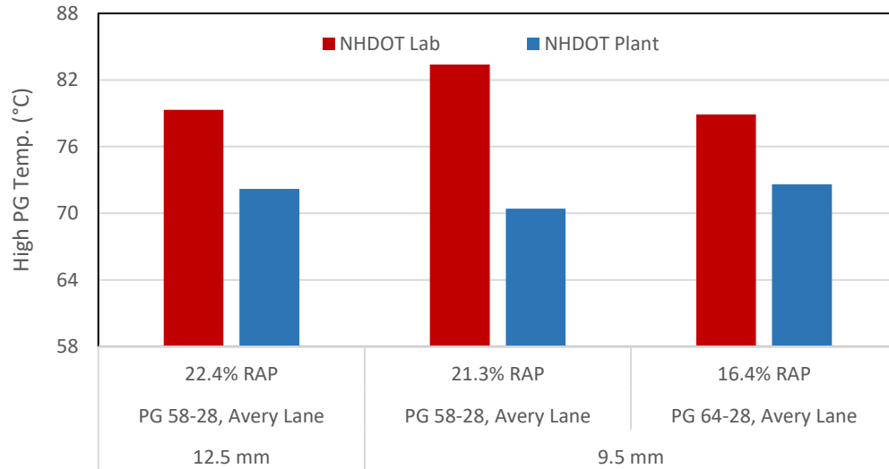
Figure 11- High PG Temperature for Hooksett Mixtures
