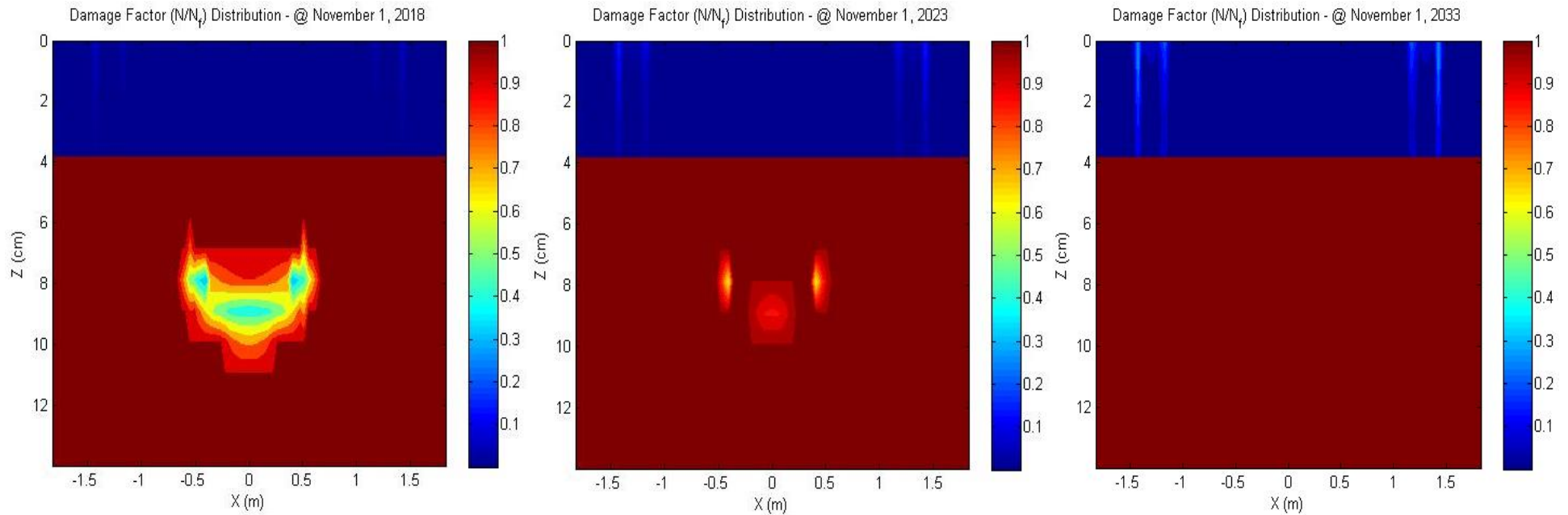
Figure 68– Plant Produced, PG 52-34, 12.5mm, 18.5% RAPRAS (Surface layer) and PG 52-34, 19mm, 20.4% RAPRAS (Binder layer) (5, 10, and 20 Years)
