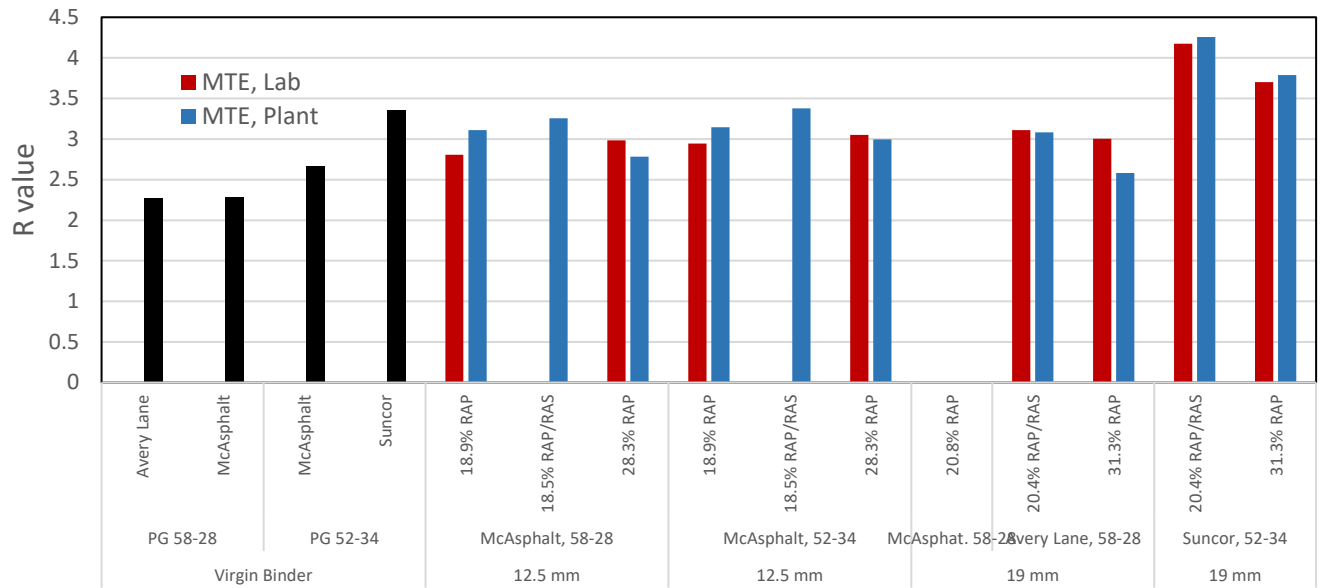
Figure 24- Rheological parameter (R-value) for different extracted and recovered binders
