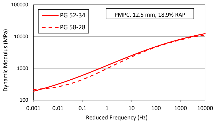
Figure 33- Comparison of Dynamic Modulus Mastercurves (12.5 mm Mixtures)
