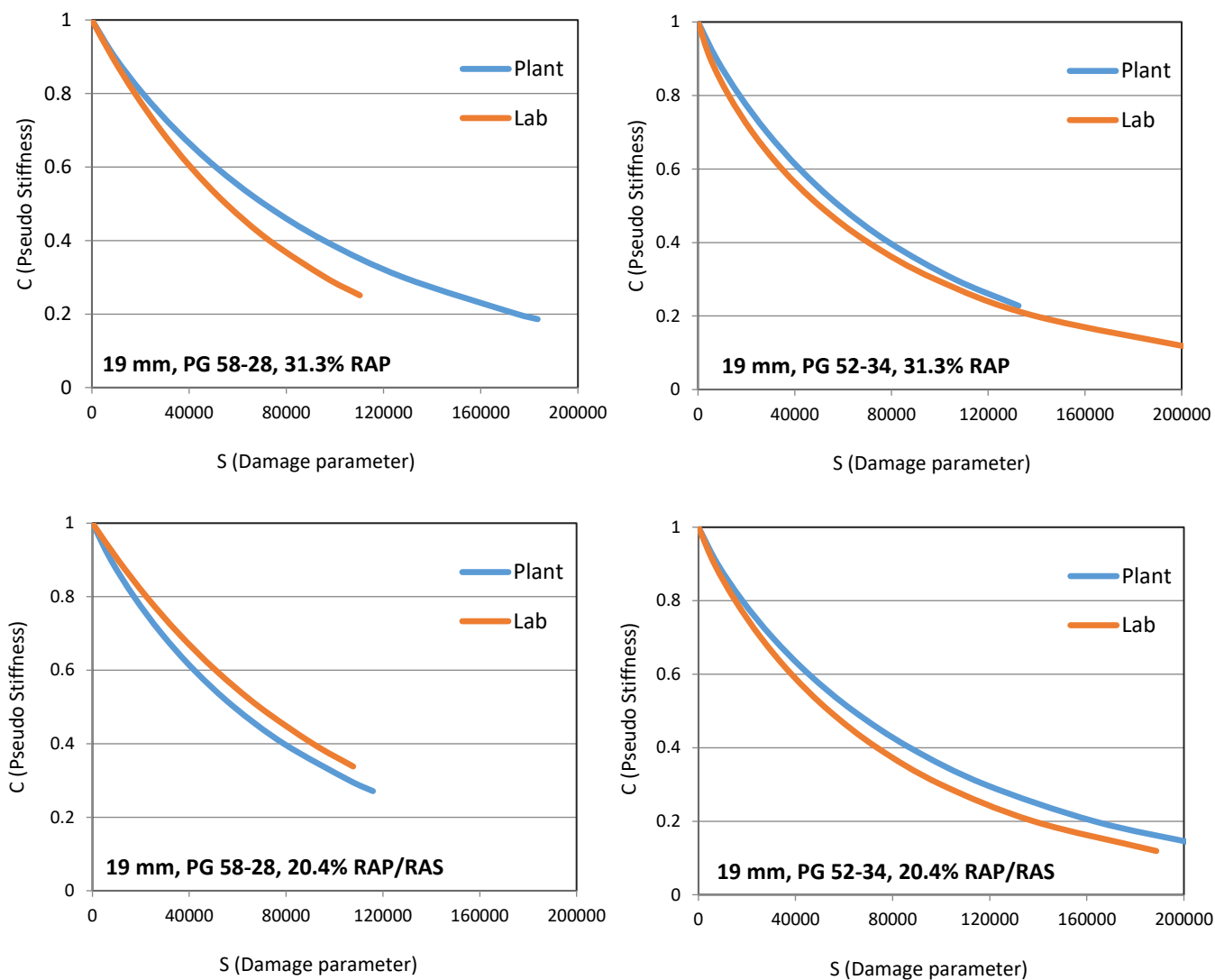
Figure 38- Damage Characteristic Curves for 19 mm, LMLC and PMPC Mixtures
