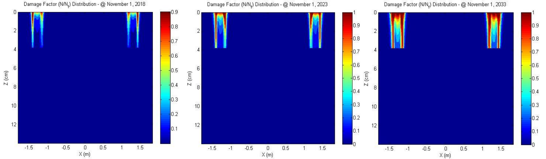
Figure 70– Lab Produced, PG 52-34, 12.5mm, 28.3% RAP (Surface layer) and PG 52-34, 19mm, 31.3% RAP (Binder layer) (5, 10, and 20 Years)
