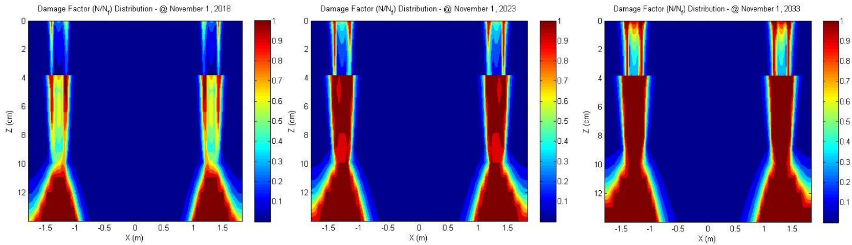
Figure 62— Lab Produced, PG 58-28, 12.5mm, 28.3% RAP (Surface layer) and PG 58-28, 19mm, 31.3% RAP (Binder layer) (5, 10, and 20 Years)
