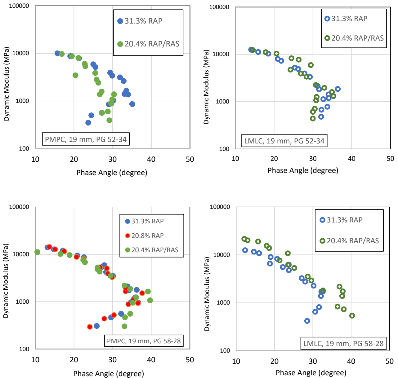
Figure 36- Black Space Diagrams of 19 mm Mixtures
