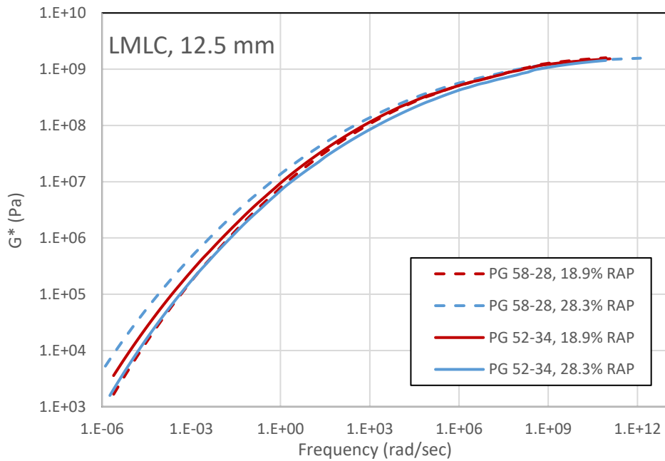
Figure 23- G^* mastercurves of extracted and recovered binders from lab produced mixtures (20hr PAV, 15° C reference temperature)
