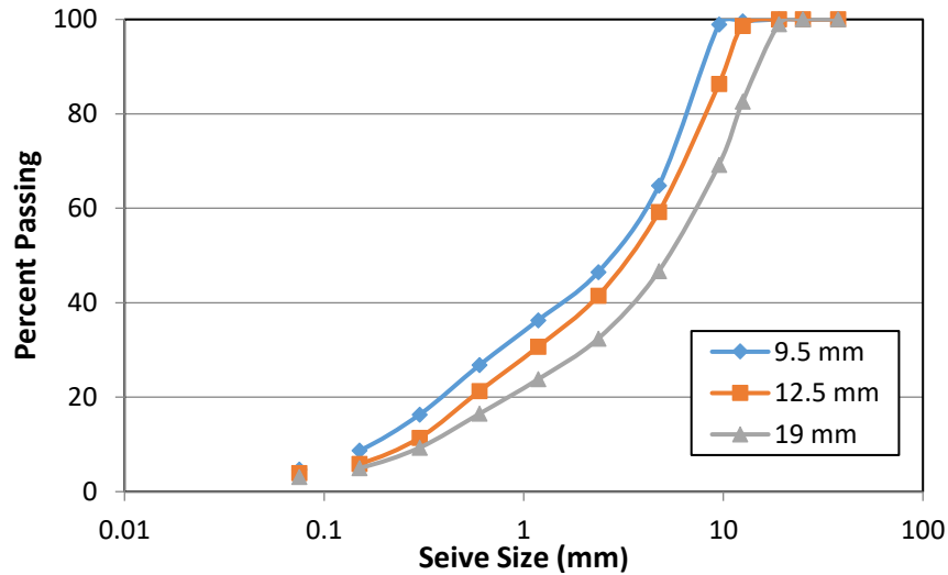
Figure 1- Aggregate Gradations
