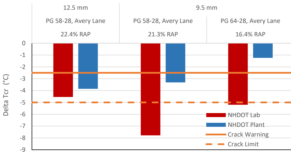
Figure 14- Delta Tcr for Hooksett Mixtures
