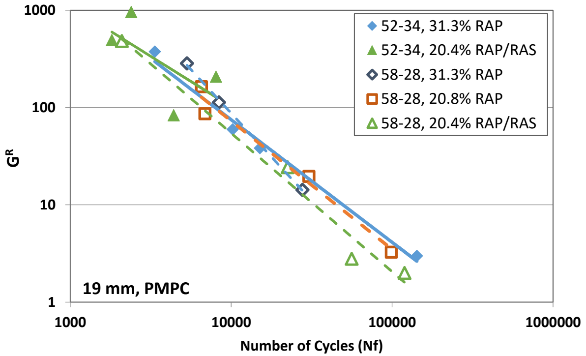
Figure 44- Fatigue Failure Diagrams of PMPC Mixtures
