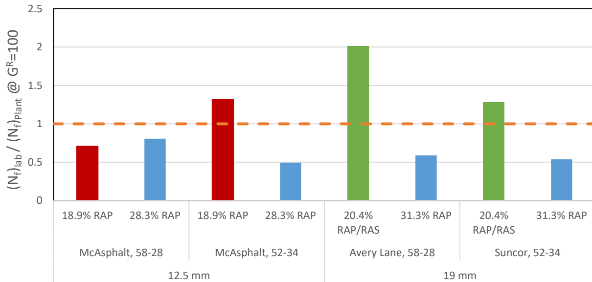
Figure 43- The ratio of (N_f)_{lab} / (N_f)_{Plant} @ G^R=100
