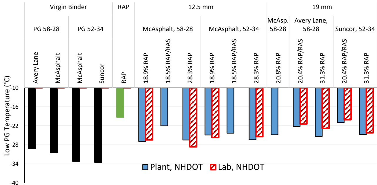
Figure 8- Low PG Temperature for Different Lebanon Binders
