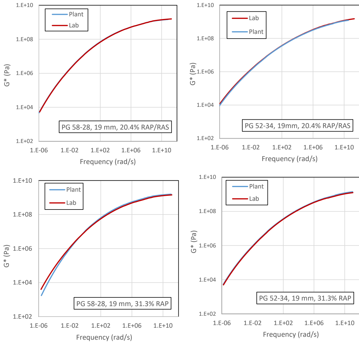
Figure 21- G^* mastercurves of extracted and recovered binders from 19.0 mm mixtures (20hr PAV, 15° C reference temperature)
