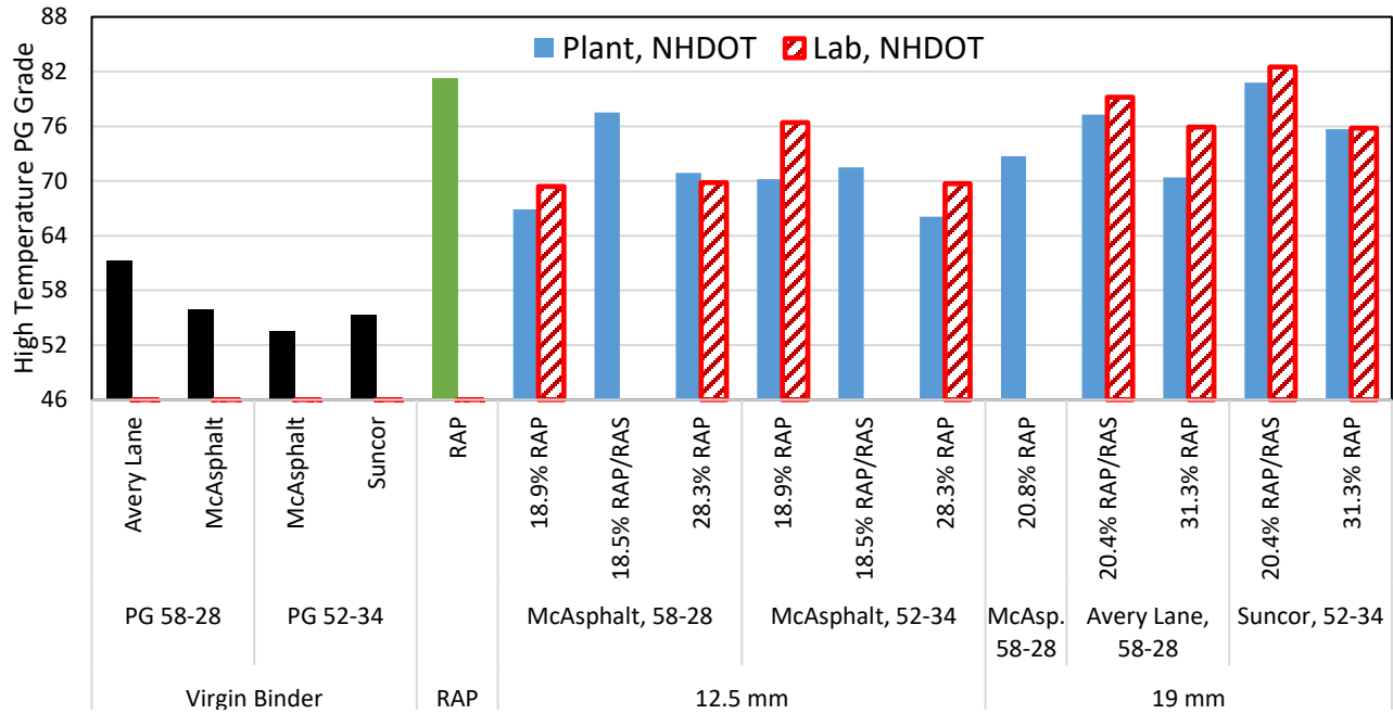
Figure 7- High PG Temperature for Different Lebanon Binders
