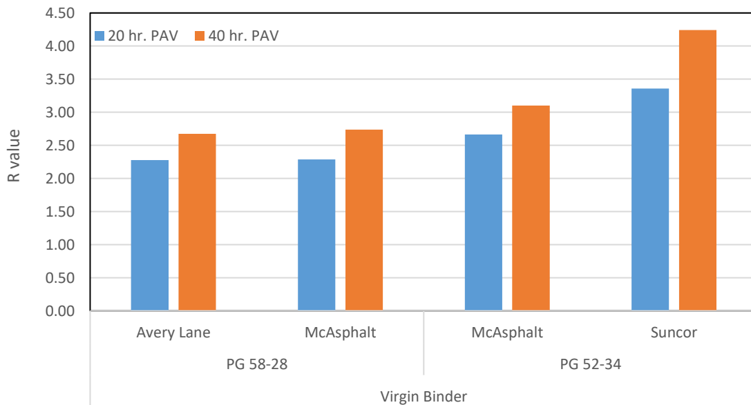
Figure 25- Rheological parameter (R-value) for virgin binders
