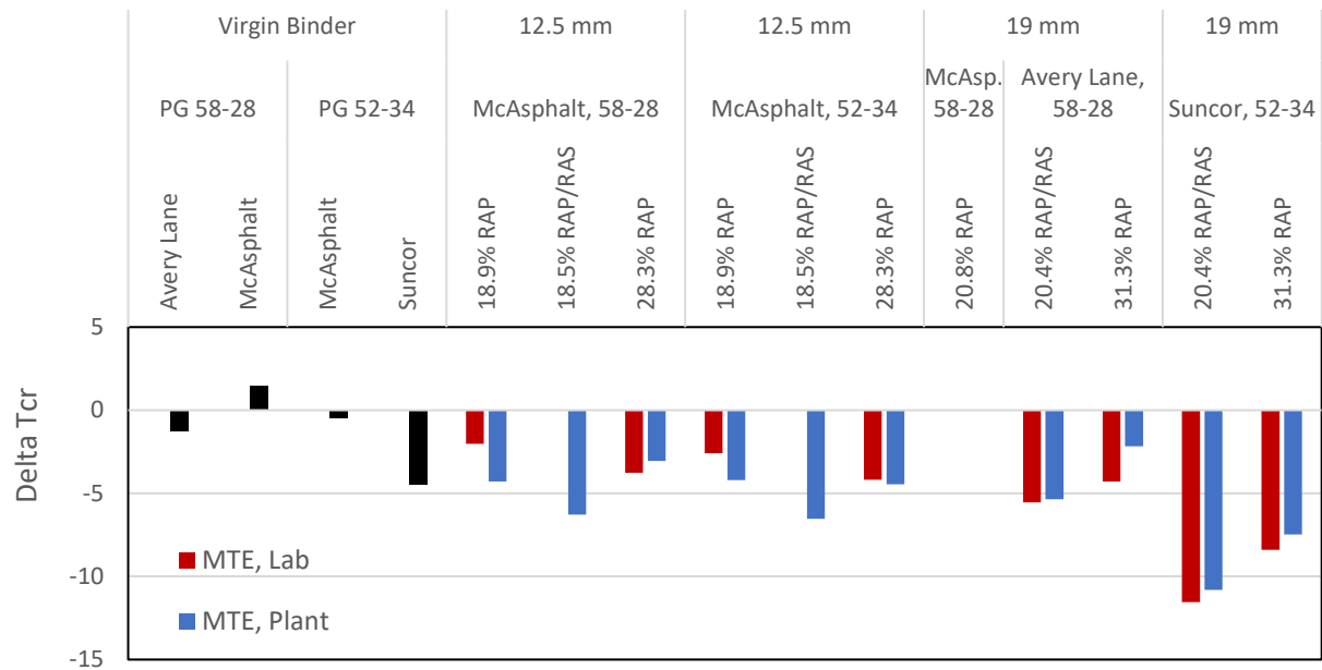
Figure 18- \Delta T_{cr} from 4 mm DSR testing (MTE), 20 hr. PAV
