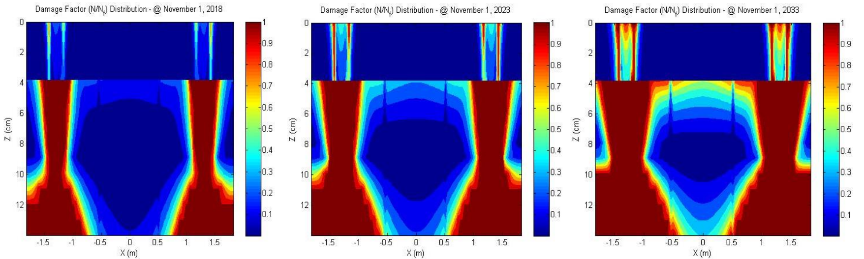
Figure 65– Lab Produced, PG 58-28, 12.5mm, 18.9% RAP (Surface layer) and PG 58-28, 19mm, 20.4% RAPRAS (Binder layer) (5, 10, and 20 Years)
