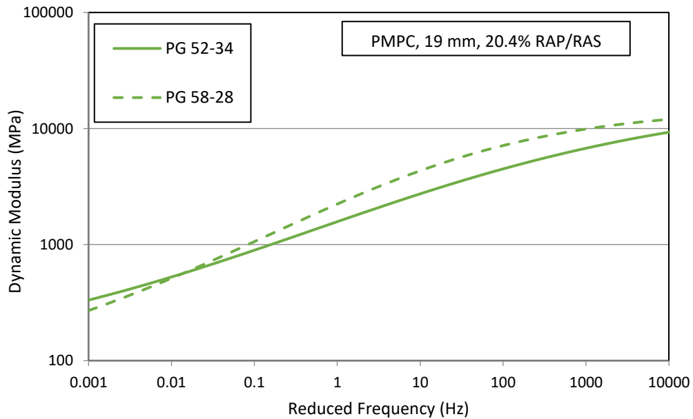
Figure 34- Comparison of Dynamic Modulus Mastercurves (19.0 mm Mixtures)
