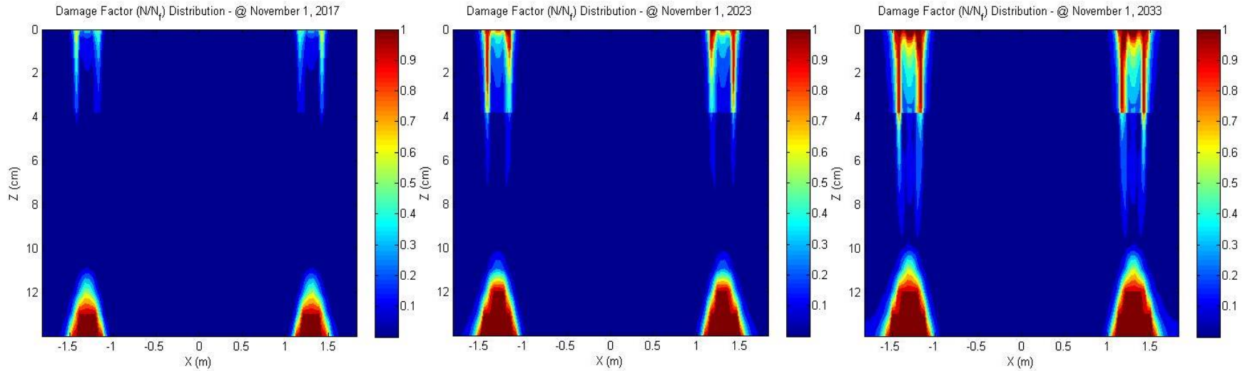
Figure 67– Lab Produced, PG 52-34, 12.5mm, 18.9% RAP (Surface layer) and PG 52-34, 19mm, 20.4% RAPRAS (Binder layer) (5, 10, and 20 Years)
