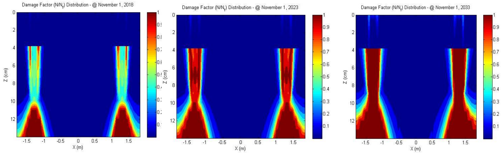
Figure 61—Plant Produced, PG 58-28, 12.5mm, 28.3% RAP (Surface layer) and PG 58-28, 19mm, 31.3% RAP (Binder layer) (5, 10, and 20 Years)
