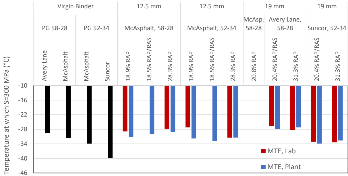
Figure 17- m and S values from 4 mm DSR testing (MTE) at 20 hr PAV
