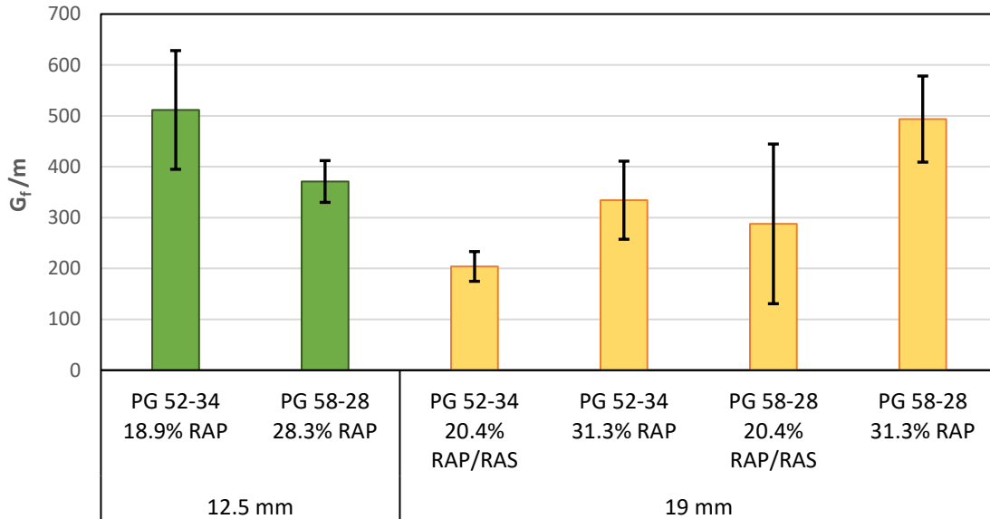
Figure 47- The Parameter of G_f/m for Different Mixtures
