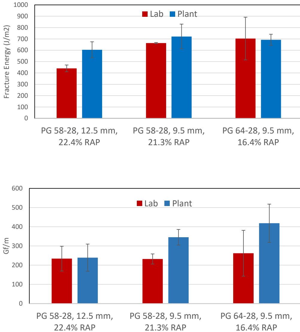
Figure 52- Fracture Energy and G_f/m for Different Hooksett Mixtures
