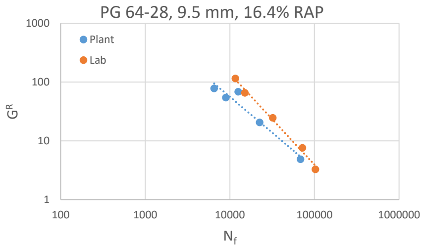
Figure 51- Fatigue Failure Criterion of Hooksett Mixtures
