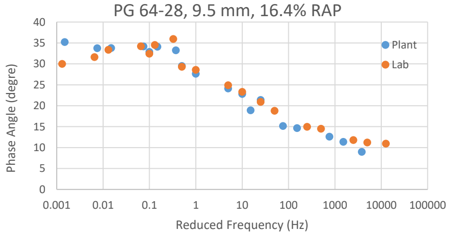
Figure 49- Phase Angle Mastercurves of Hooksett Mixtures
