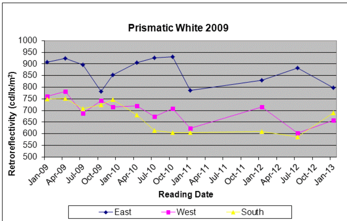
Figure 2: 2009 reflectivity measurements on white sign sheeting based on facing direction.
