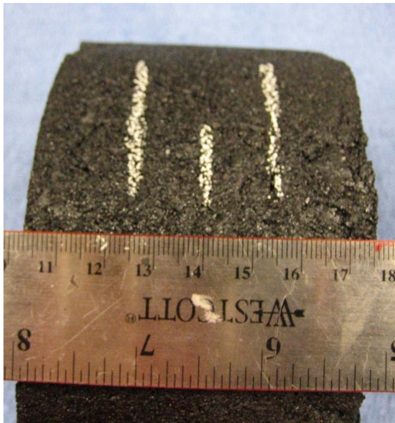
Figure 2.2: Gyratory Compacted Sample Marked for Cutting
