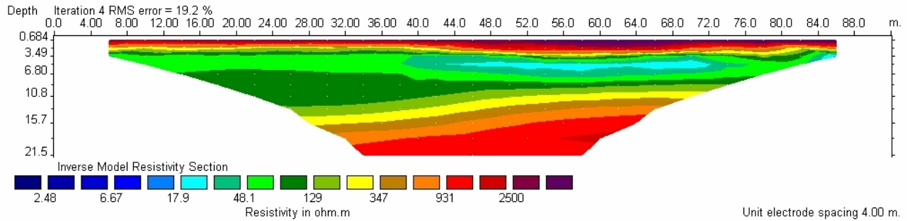
Figure 14: Dipole-Dipole array looking for 1.5-meter metal pipe at a depth of 18 meters.
