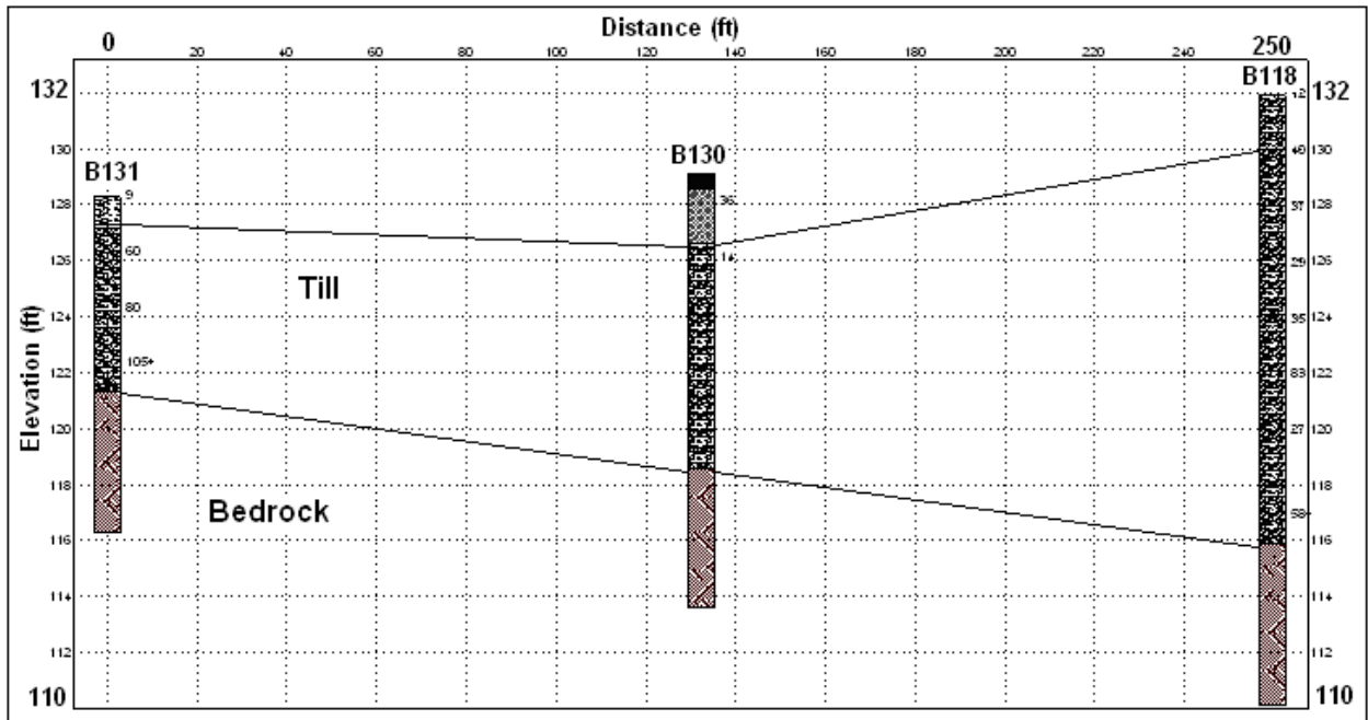
Figure 10: Fence diagram of test borings along a section of Old Country Road.
