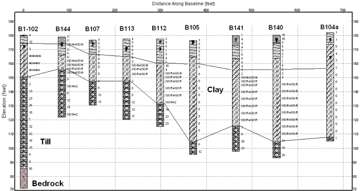
Figure 3: Fence diagram of test boring logs from Exit 12 southbound on-ramp
