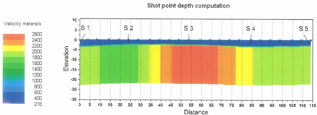
Figure 15: Typical seismic refraction profile along southern side of roadway
