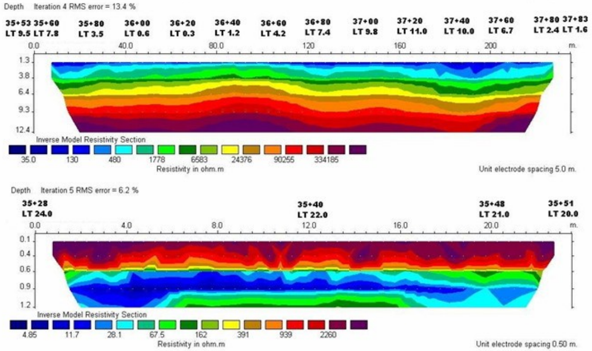
Figure 18: Resistivity profiles along the southern & northern sides of the road.
