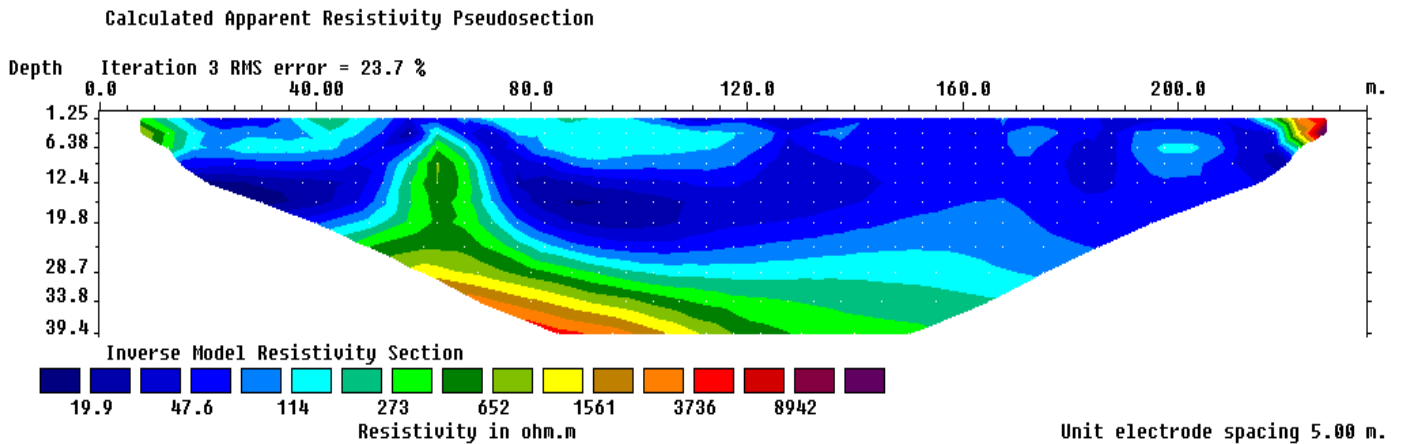
Figure 2: Wenner-Schlumberger resistivity array
