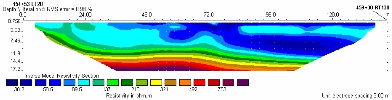
Figure 5: Wenner-Schlumberger array
