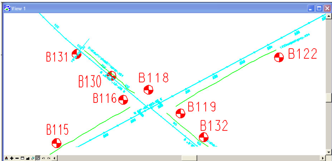
Figure 9: Plan of Old Country Rd & NH Route 125 showing test borings & seismic lines.
