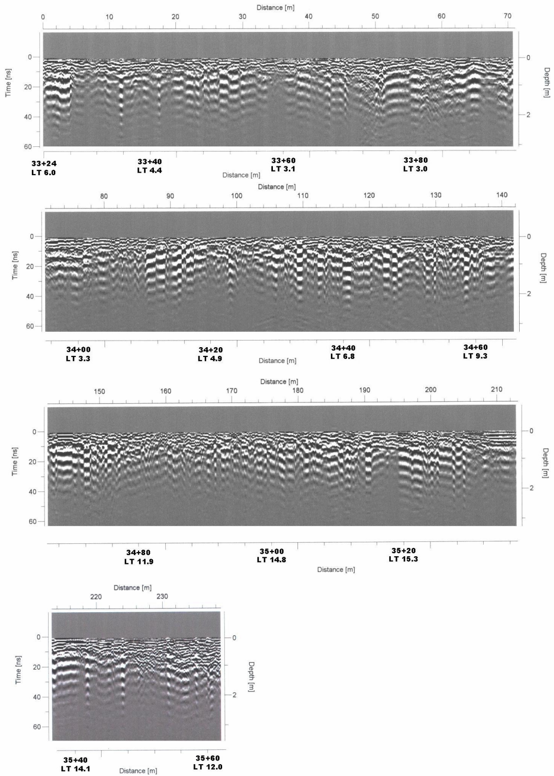
Figure 20: GPR profiles using 500 MHz antenna.
