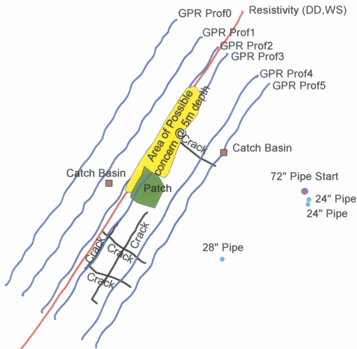
Figure 12: Geophysical and GPS survey of project.
