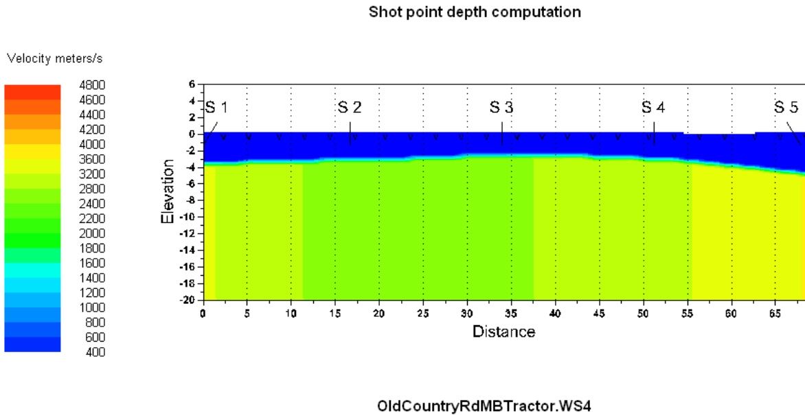
Figure 8: Seismic velocity profile along 1 section of Old Country Road.
