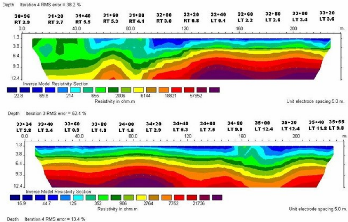
Figure 17: Resistivity profiles along the southern side of the road.
