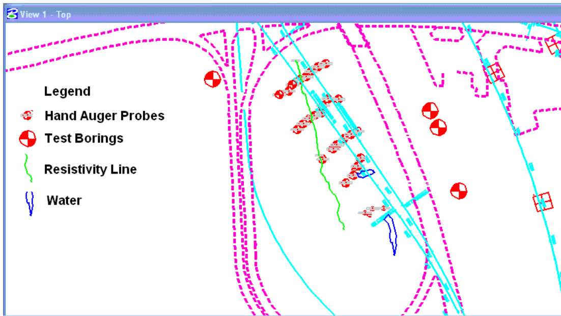
Figure 6: Exit 3 ramp alignments, location of hand auger probes & resistivity line.
