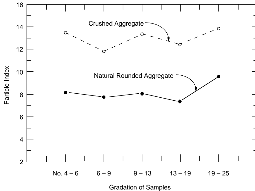
Figure 5. Comparison of particle index values for rounded and crushed coarse aggregates.
