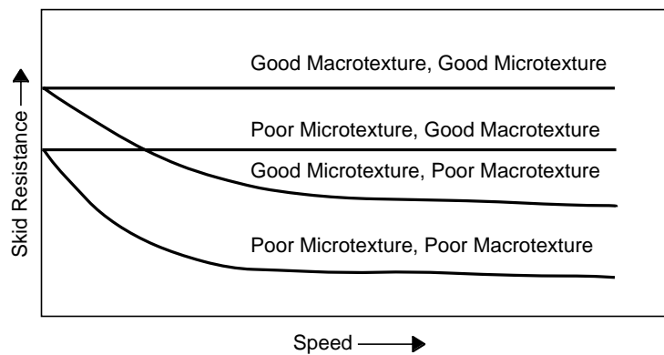
Figure 14. Correlation between macrotexture, microtexture, skid resistance, and speed (Tremblay 1995).
