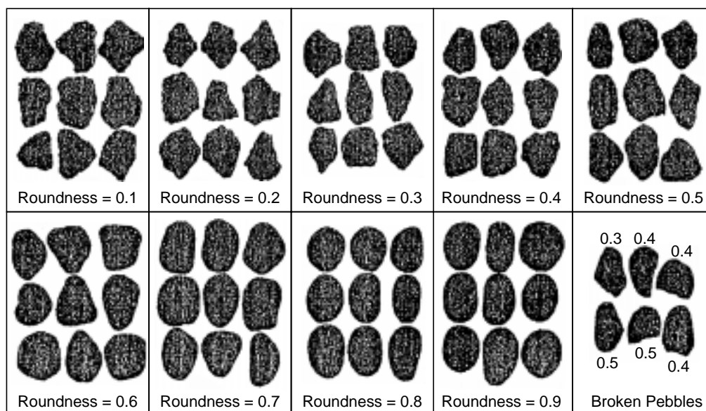
Figure 3. Roundness chart for 16- to 32-mm aggregates.
