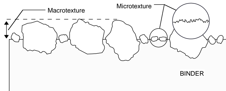
Figure 13. Road surfacing textural characteristics (Tremblay 1995).
