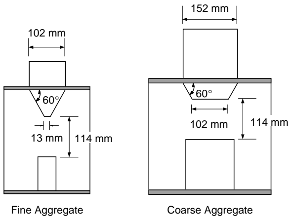
Figure 10. Test apparatus for ASTM C 1252 and modified ASTM C 1252.
