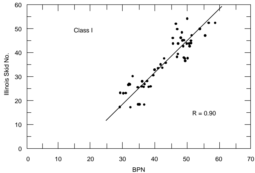
Figure 21. Relationship between British pendulum number and Illinois skid trailer number.
