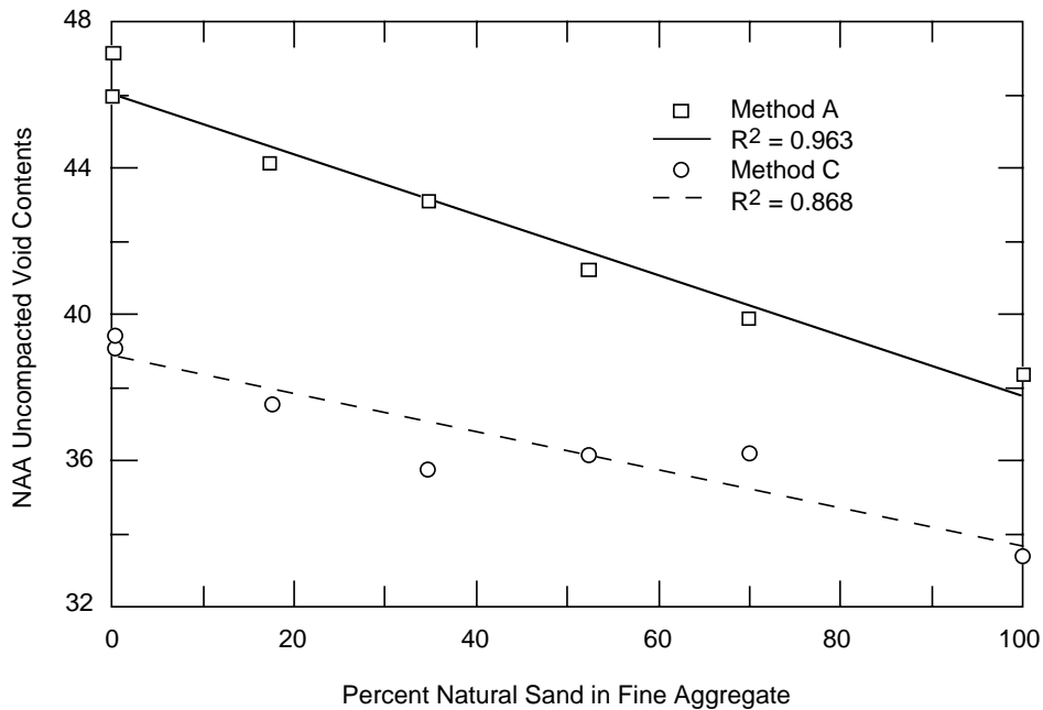
Figure 9. NAA particle shape and texture void contents vs. percent natural sand in fine aggregate
