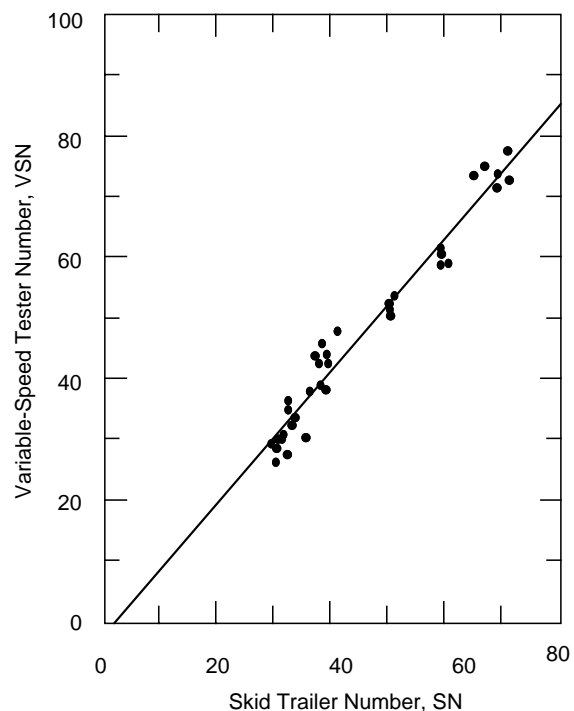
Figure 22. Correlation between variable-speed number and skid trailer number at 40 mph.
