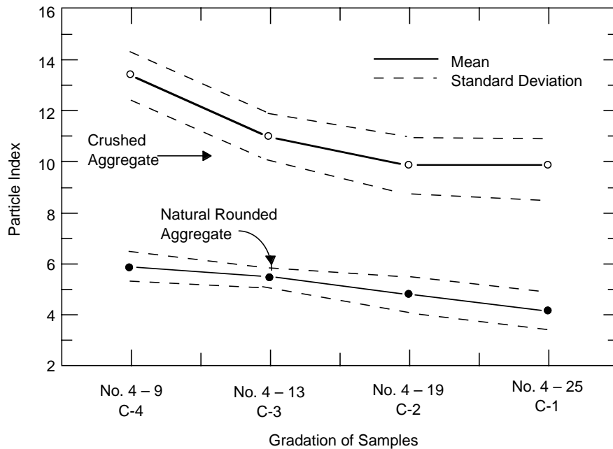
Figure 6. Particle index for different aggregate gradations.
