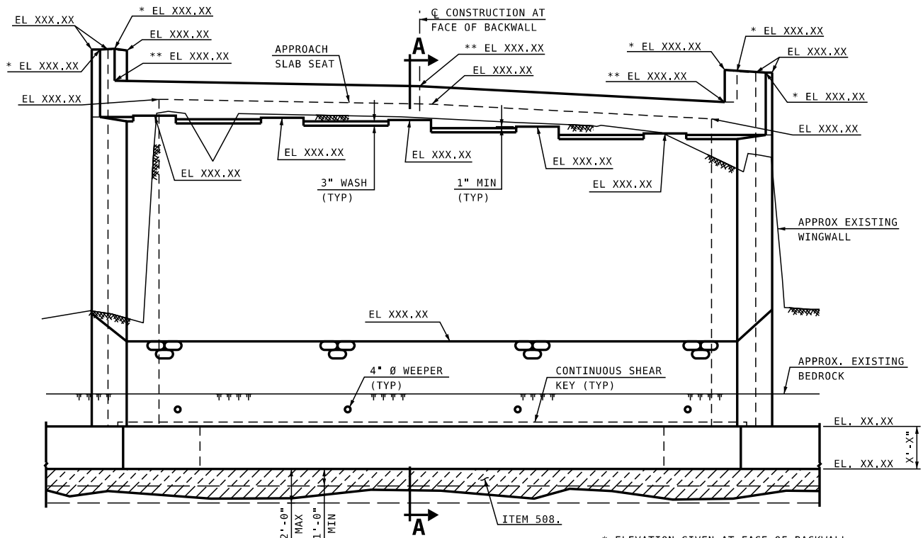
TYP ABUTMENT ELEVATION
