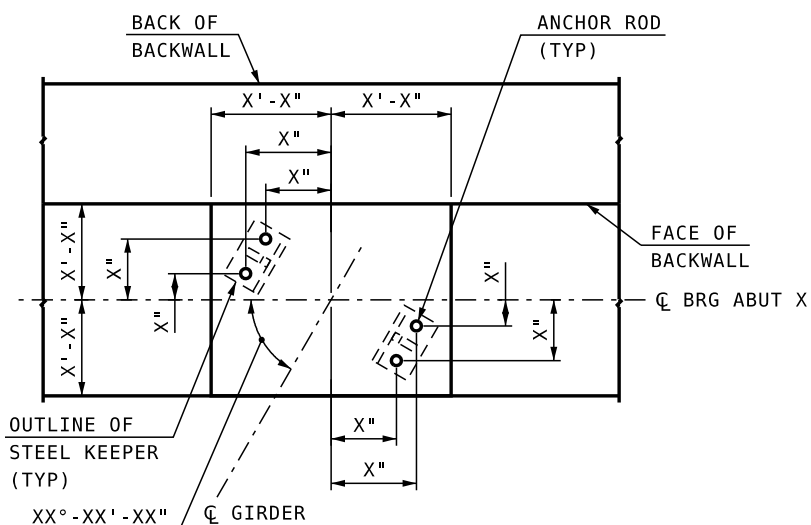
ANCHOR ROD LAYOUT
