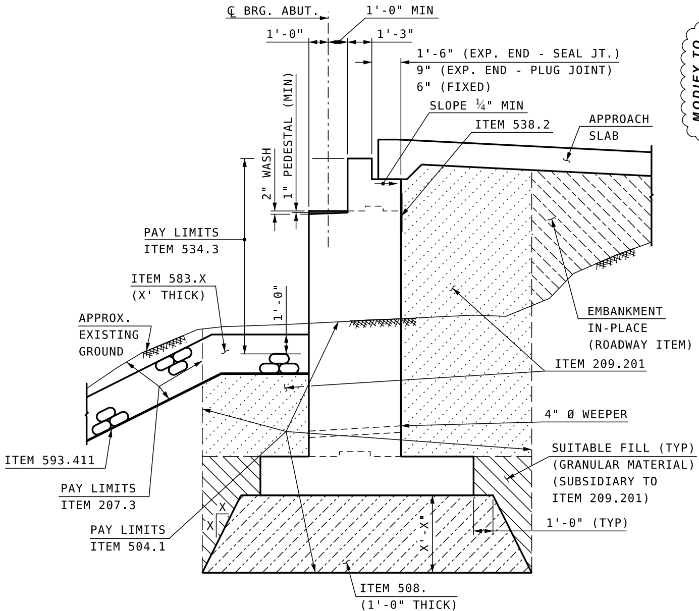
TYPICAL ABUTMENT SECTION (DECK OVER BACKWALL)
