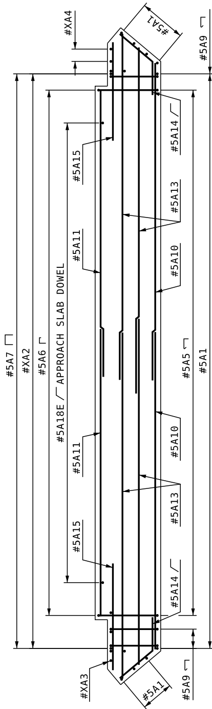
SECTION C-C
