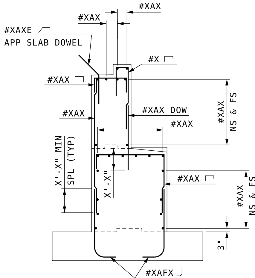
TYPICAL REINF. ABUT. SECTION (DECK OVER BACKWALL)
