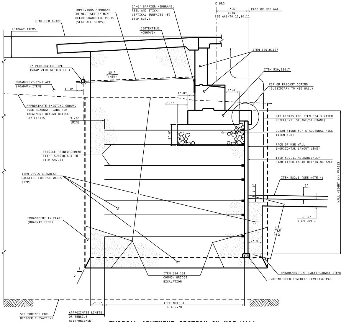
TYPICAL ABUTMENT SECTION ON MSE WALL
